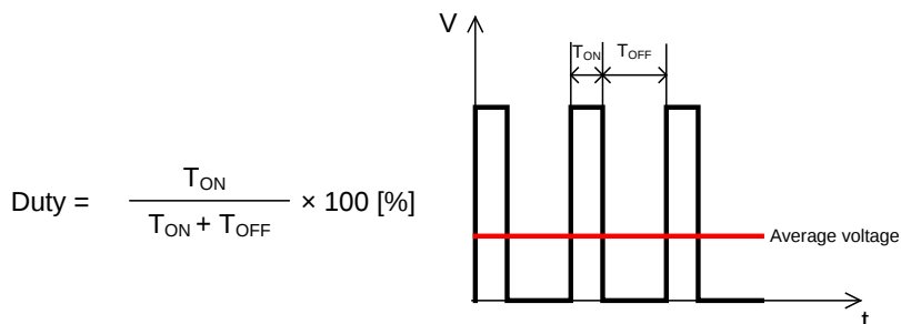
Figure 3-2 PWM control
