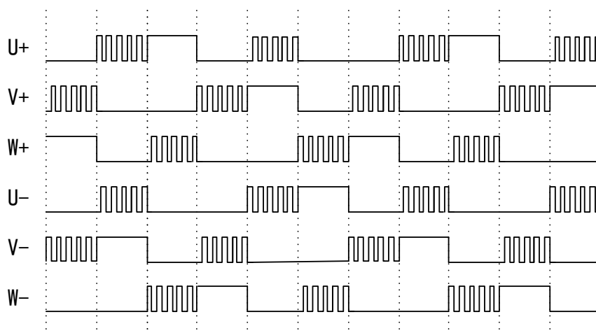
Figure 3-3 Complimentary first 60 degrees chopping
