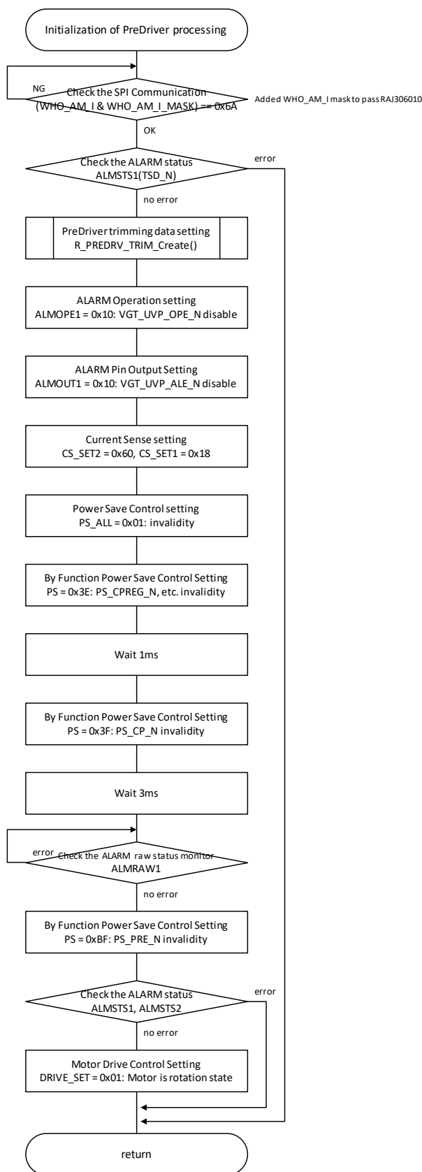
Figure 3-8 Flow chart (Initialization of PreDriver processing)
