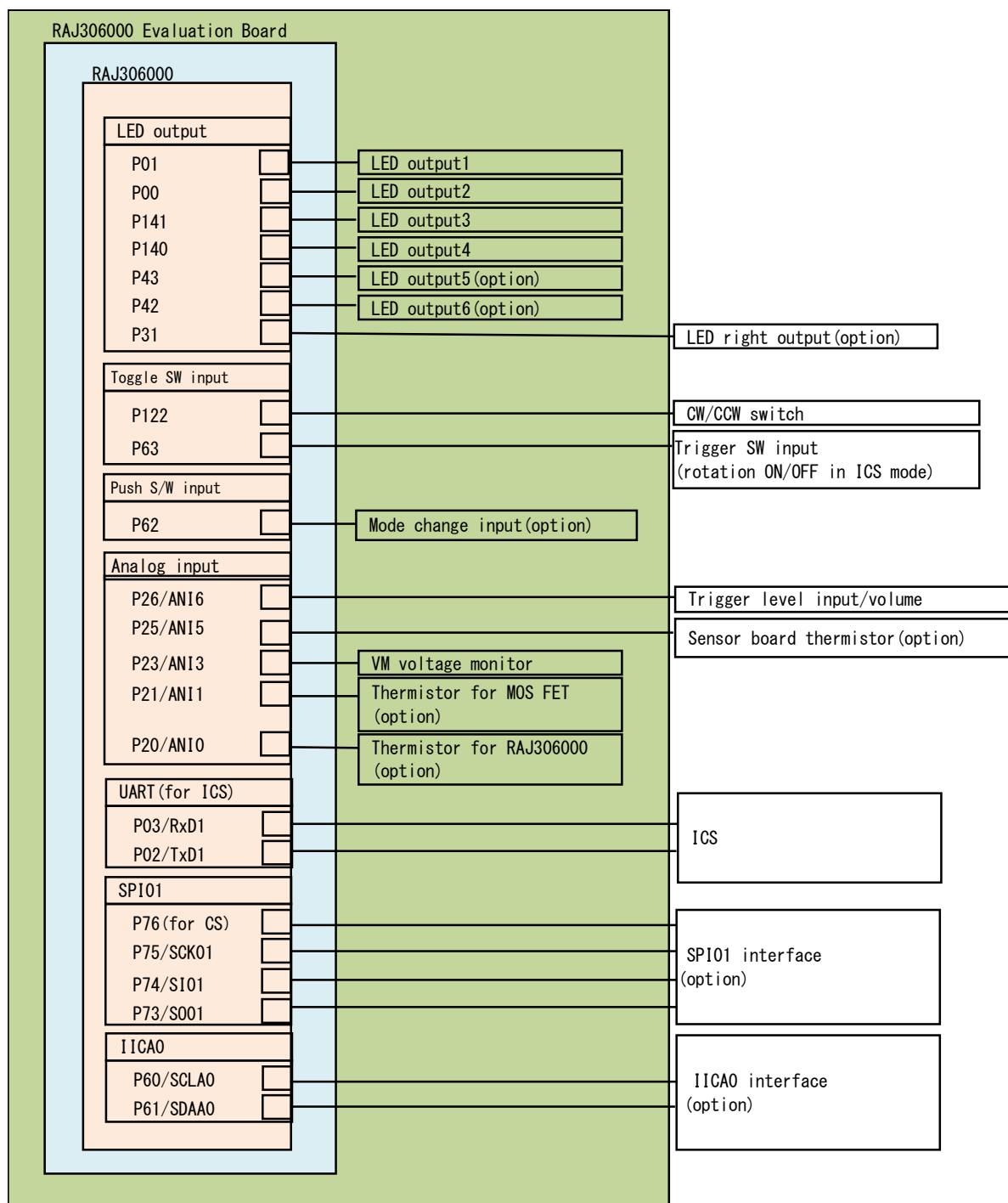
Figure 2-3 Hardware Configuration Diagram (RL78/G1F, Peripheral)
