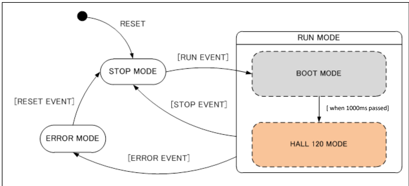
Figure 3-4 State Transition Diagram
