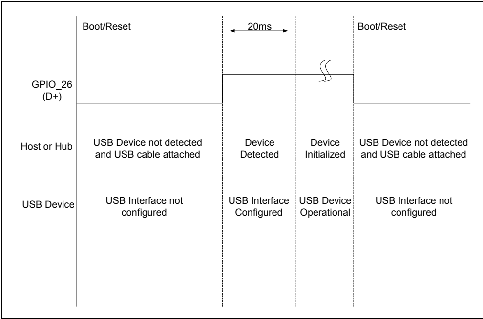
Figure 2 Timing Diagram of USB Configuration
