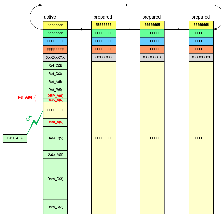
Figure 4-16 EEL pool after WRITE command (normal example).
