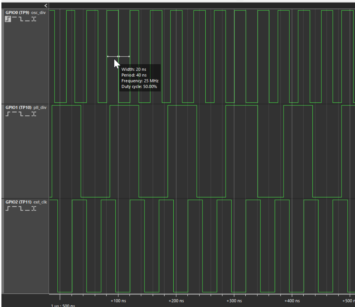
Figure 4: Waveform using External Clock
