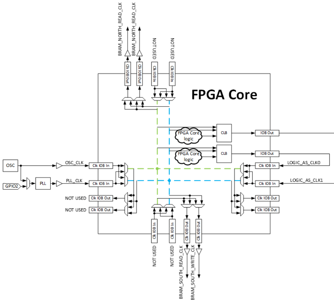
Figure 1: Clock Network
