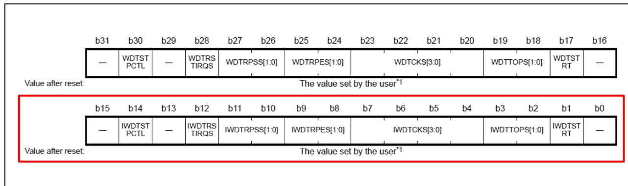
Figure 2.10 Option Function Select Register 0 (OFS0)
