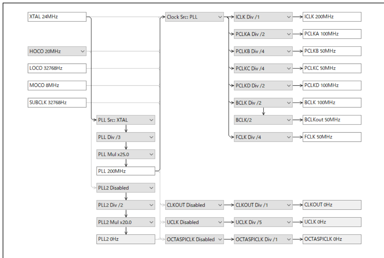
Figure 3.1 Clock Configuration
