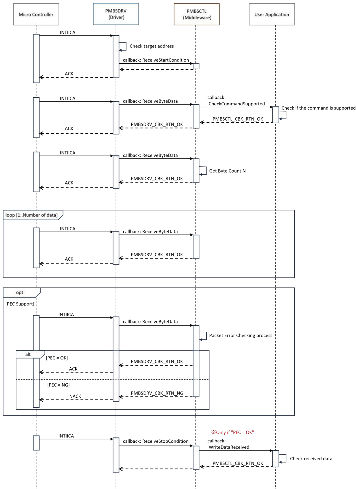
図 5-4 Block Write sequence
