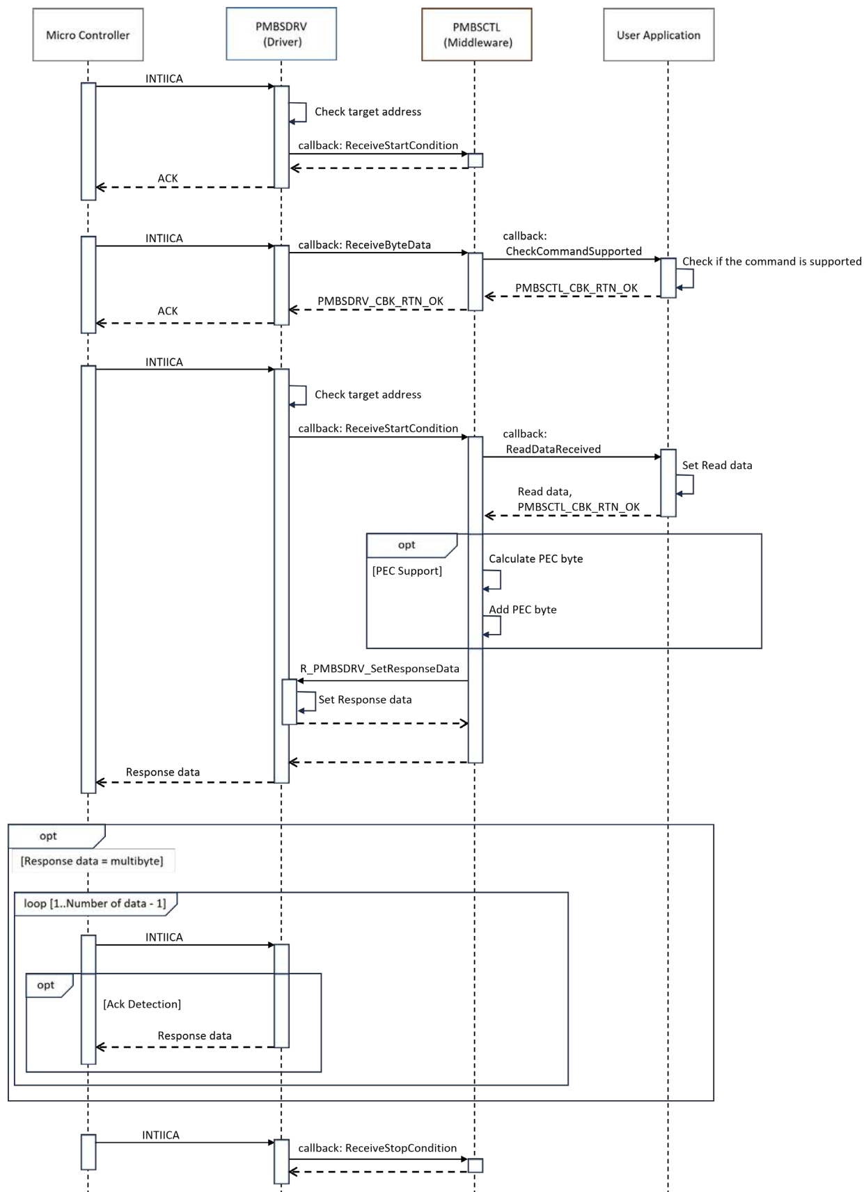
図 5-3 Read sequence
