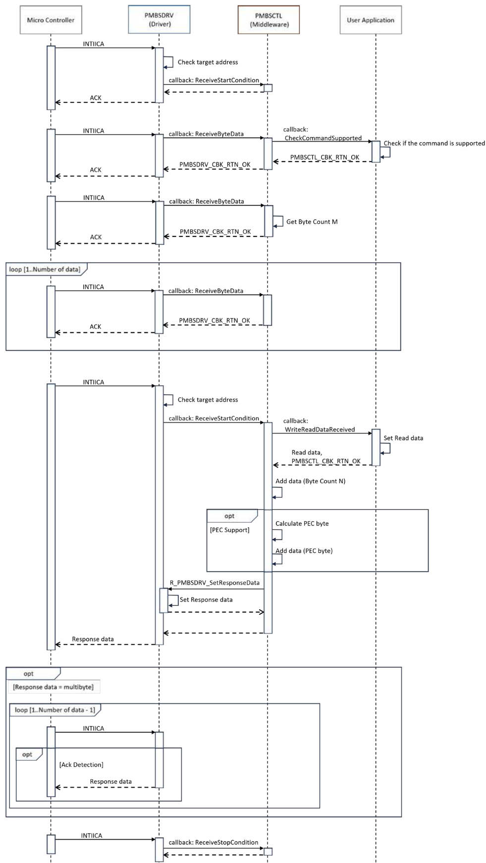
図 5-6 Block Write-Block Read Process sequence
