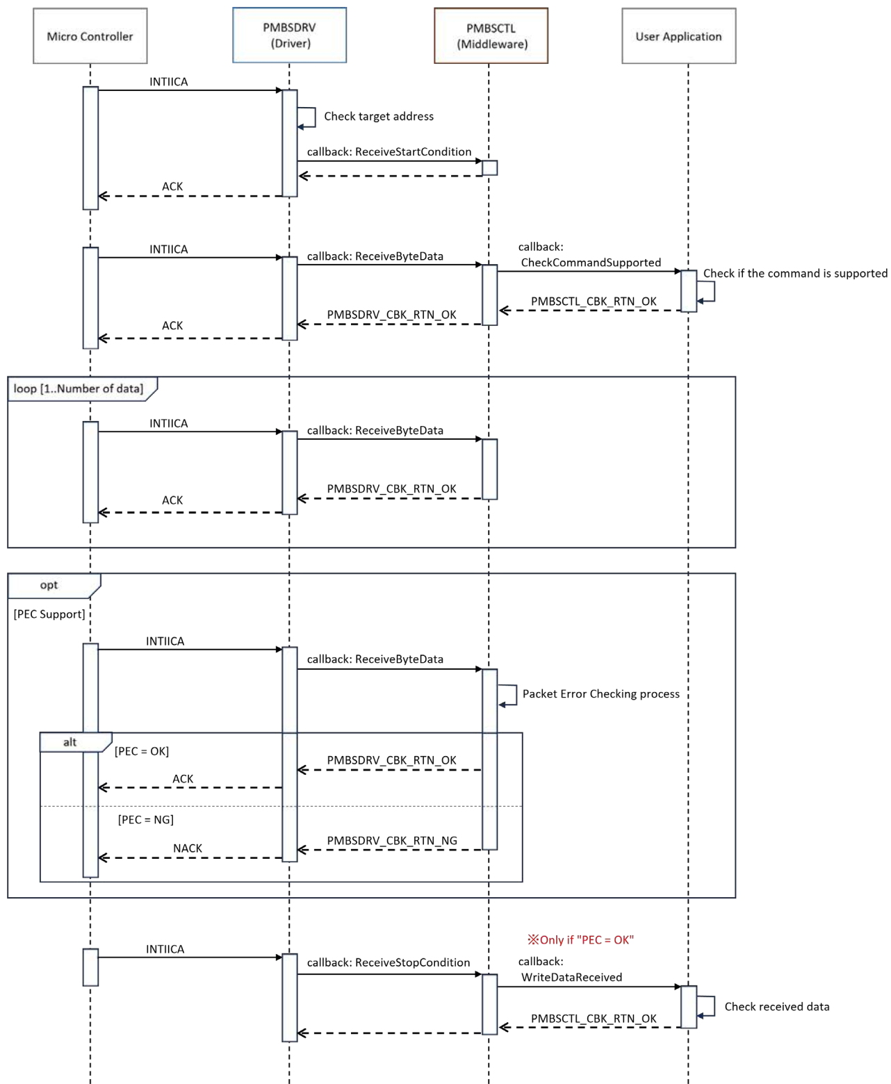
図 5-2 Write sequence
