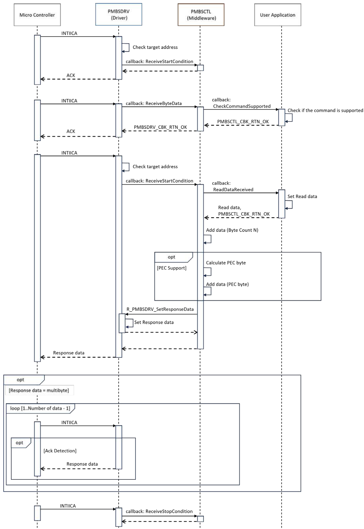
図 5-5 Block Read sequence
