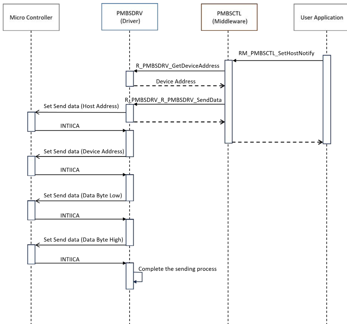
図 5-8 SMBus Host Notify sequence
