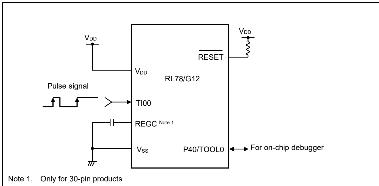
Figure 4.1 Hardware Configuration
