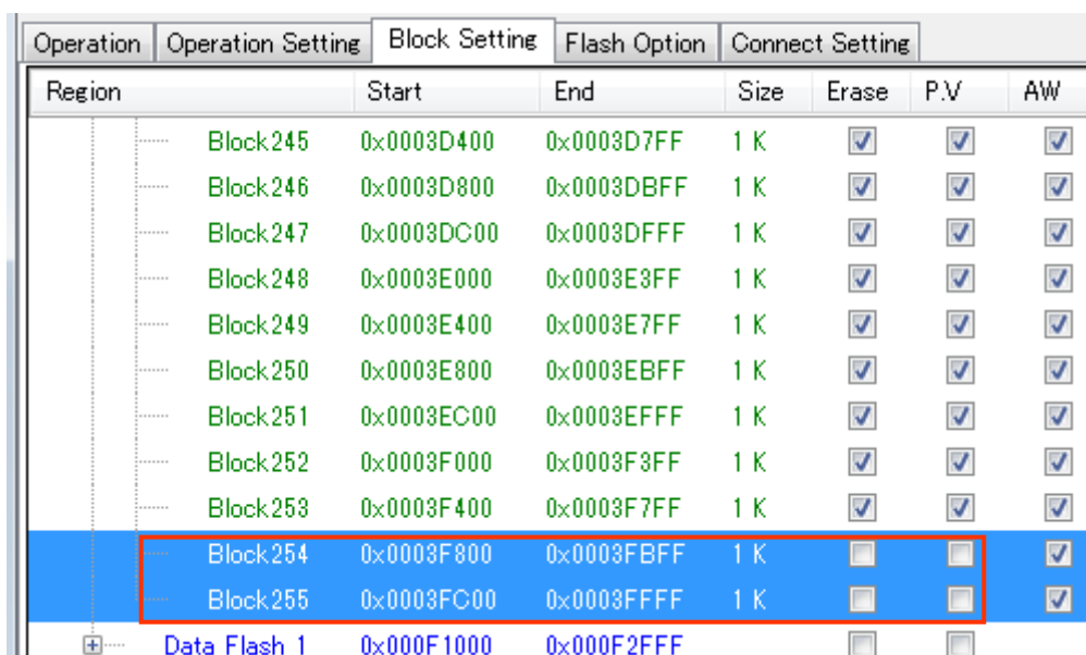
Figure 8-2 Setting of RFP V3 (2)
