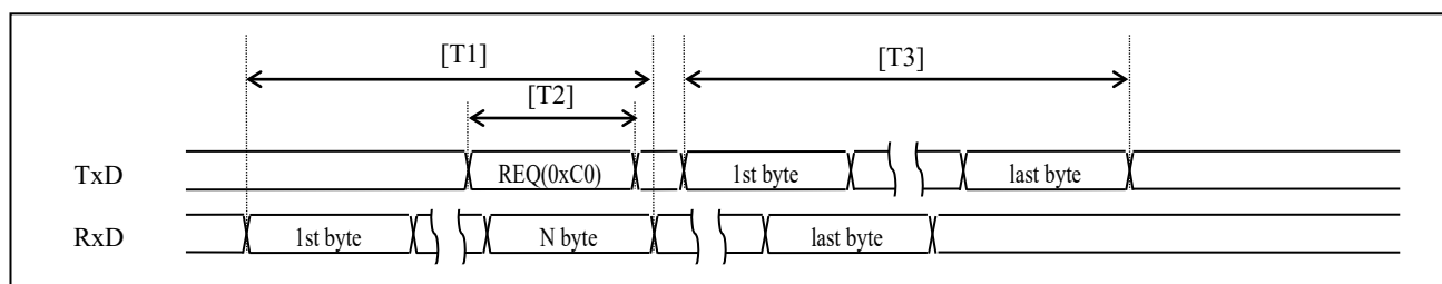
Figure 6-4 Transmit timing chart (Host MCU) (While the Module transmitting)
