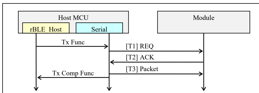
Figure 6-6 Transmit Sequence (Host MCU)
