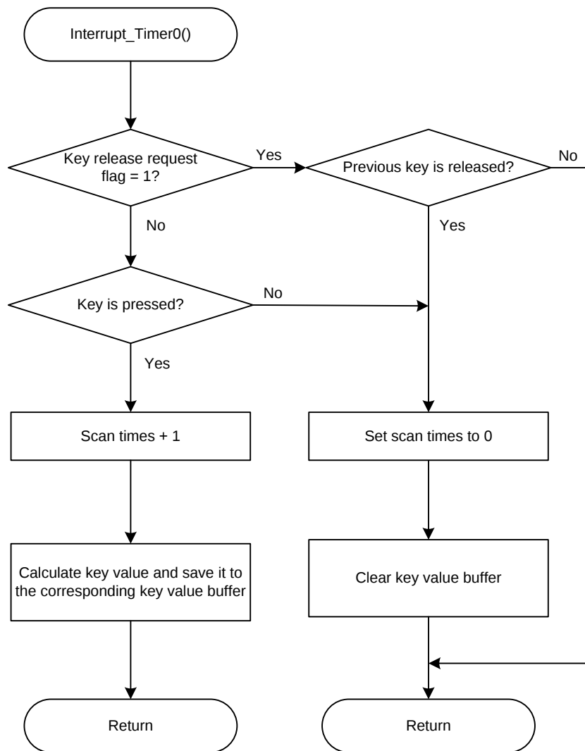
Figure 5.3 Flow Chart of KEY&LED Scan (2/2)
