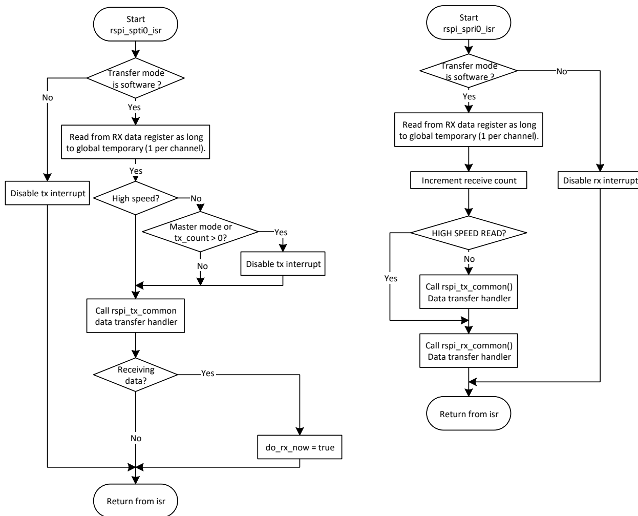
Figure 1-4. Common interrupt handler algorithm.
