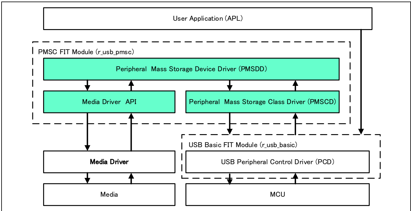
Figure 2-1 Module Configuration
