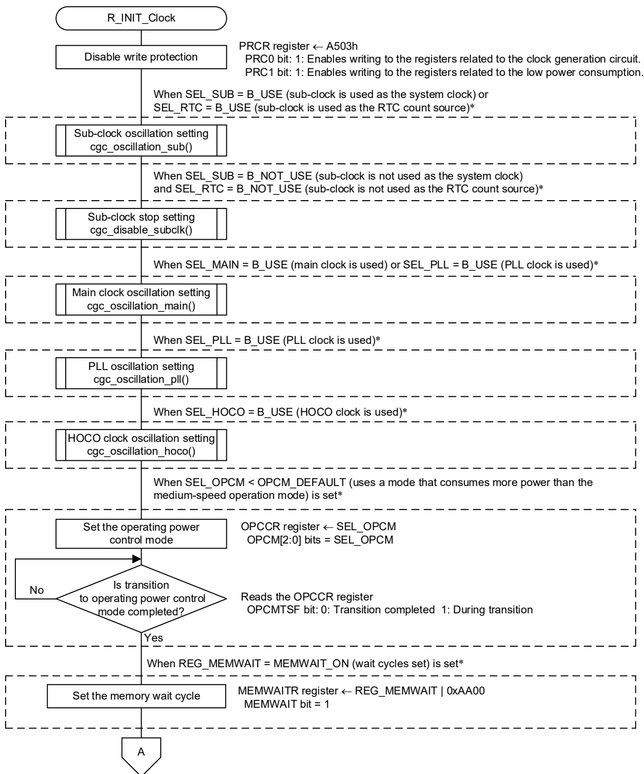
Figure 4.5 Clock Initialization (1/2)
