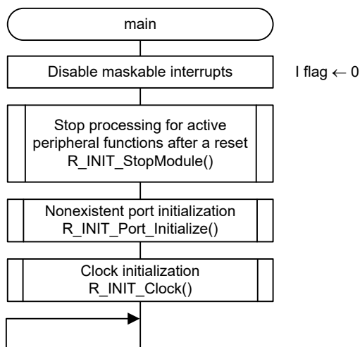
Figure 4.2 Main Processing
