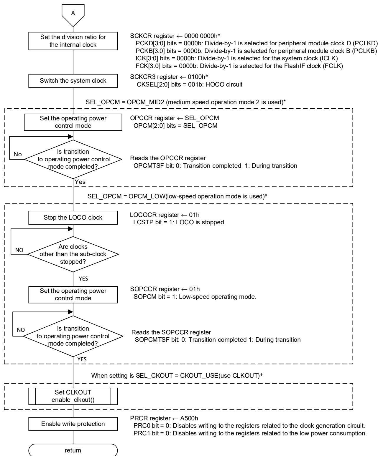
Figure 4.6 Clock Initialization (2/2)
