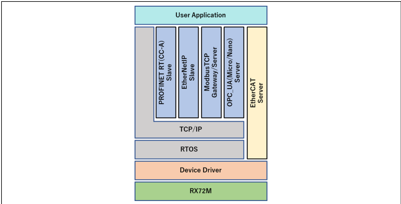
Figure 2.1 overall structure of protocol stack software for RX72M
