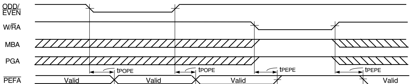
Figure 11. ODD/EVEN, W/RA, MBA, and PGA to \overline{\text{PEFA}} Timing
