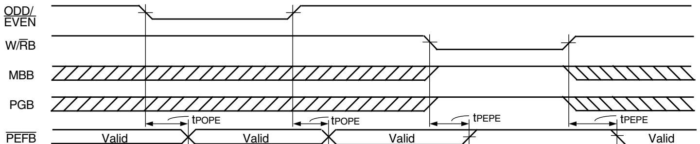
Figure 12. ODD/EVEN, W/RB, MBB, and PGB to \overline{\text{PEFB}} Timing
