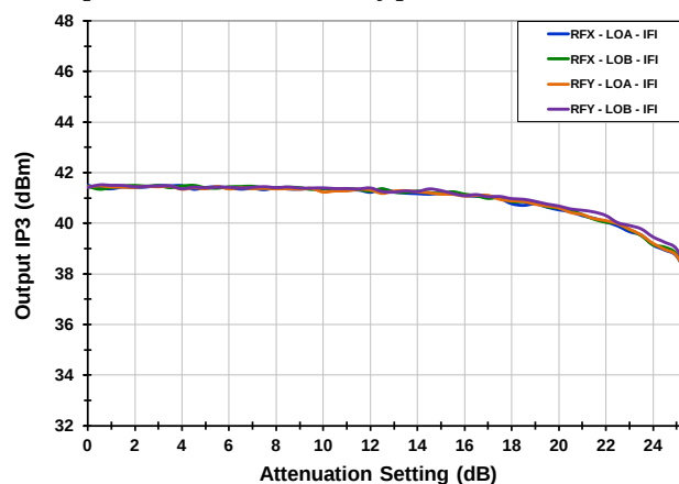
IP3 O [1.0 GHz RF, HiSide Inj.]
