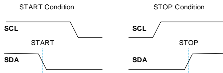
Figure 5. START and STOP Condition Waveform
