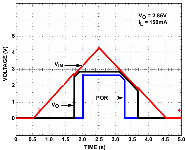
FIGURE 12. POWER-UP/POWER-DOWN
