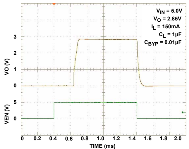
FIGURE 13. TURN-ON/TURN-OFF RESPONSE
