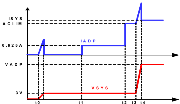
FIGURE 40. NO BATTERY SOFT-START WITH ISYS > ACLIM
