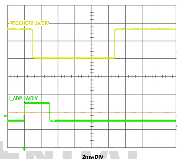
FIGURE 19. ACPROCHOT# ASSERTION. ACPROCHOT = 2.048A , PROCHOTDEBOUNCE = 1ms , PROCHOTDURATION = 10ms
