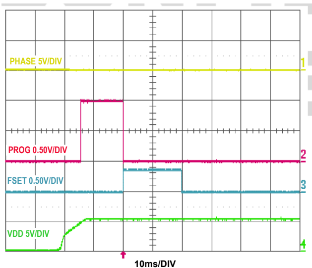
FIGURE 8. POWER-UP, READ PROG, AND FSET RESISTORS
