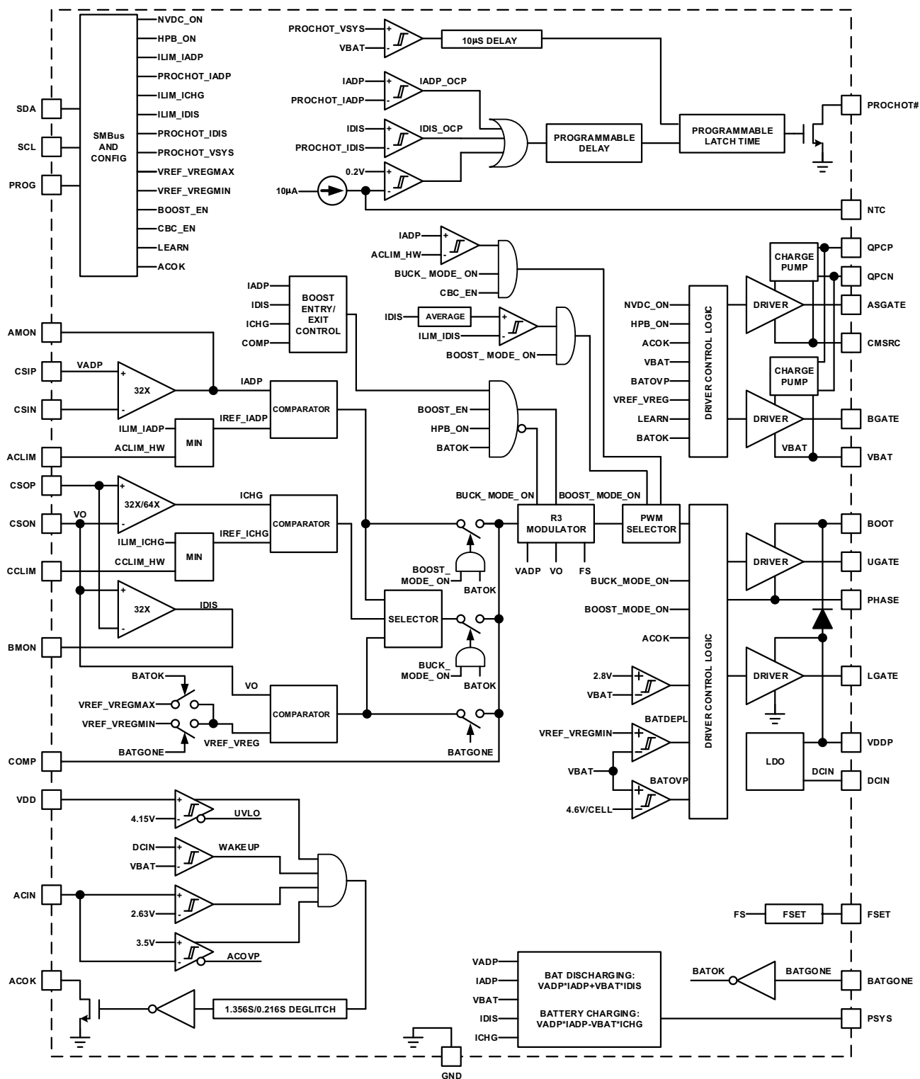
FIGURE 7. BLOCK DIAGRAM
