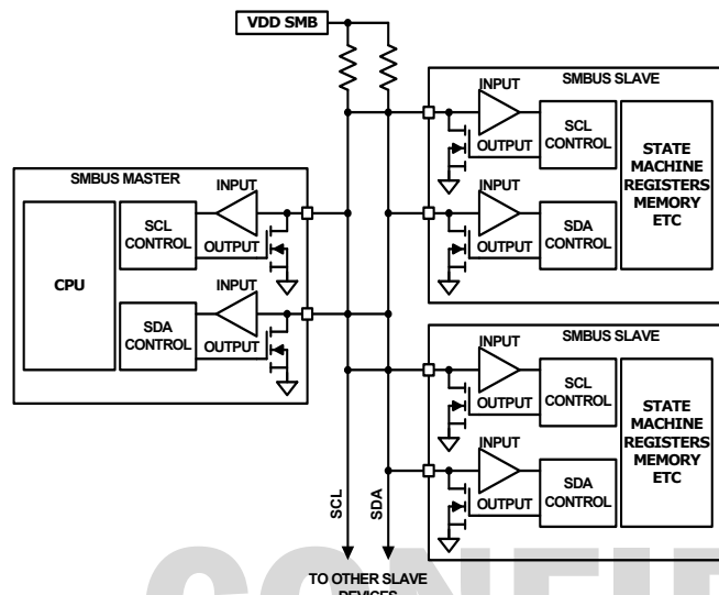
FIGURE 26. GENERAL SMBus ARCHITECTURE
