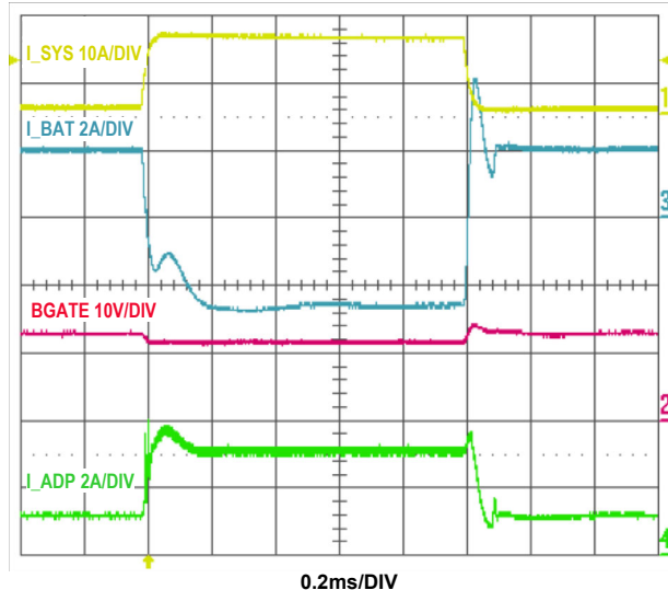
FIGURE 13. NVDC: CHARGING CURRENT LIMIT LOOP AND TURBO MODE TRANSITION. V_{ADP} = 20V , ADAPTERCURRENTLIMIT1 = 3.072A , V_{BAT} = 7V , MAXCHARGEVOLTAGE = 8.192V , CHARGECURRENT = 2.016A , 1A-12A SYSTEM LOAD STEP
