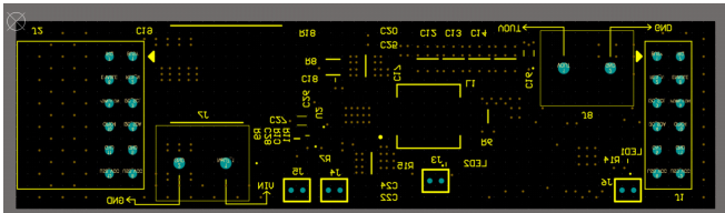
Figure 9. Top Overlay
