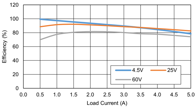
Figure 17. Efficiency
