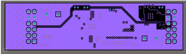
Figure 13. Layer 4 (Signal)
