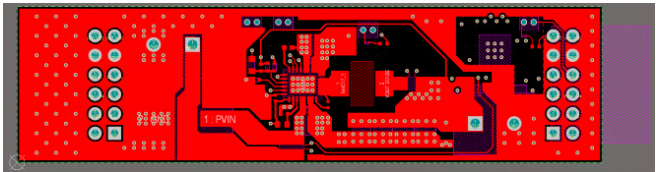
Figure 10. Top Layer
