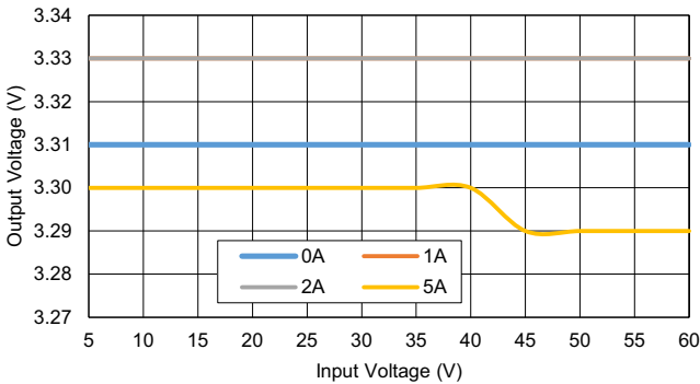
Figure 19. Line Regulation
