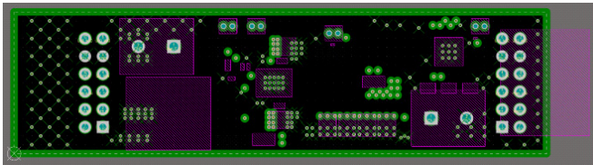
Figure 11. Layer 2 (GND)
