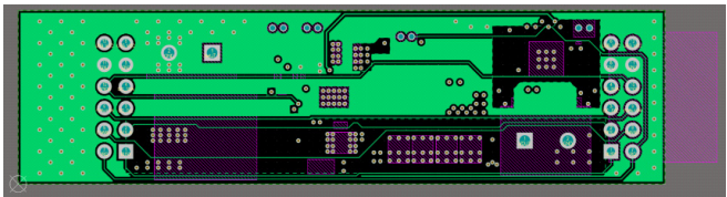
Figure 12. Layer 3 (Signal)
