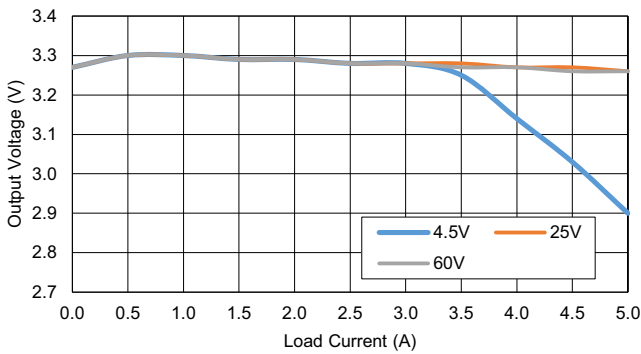
Figure 18. Load Regulation
