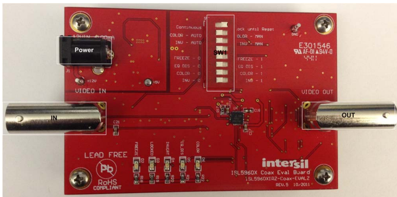
FIGURE 1. TOP VIEW OF EVALUATION BOARD
