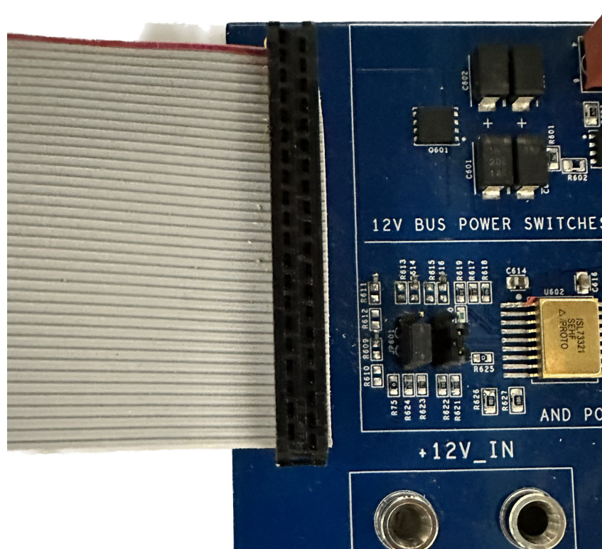
Figure 4. ISL73141VMREFEV1Z Evaluation Board with Vorago VA41620 MCU Evaluation Board
