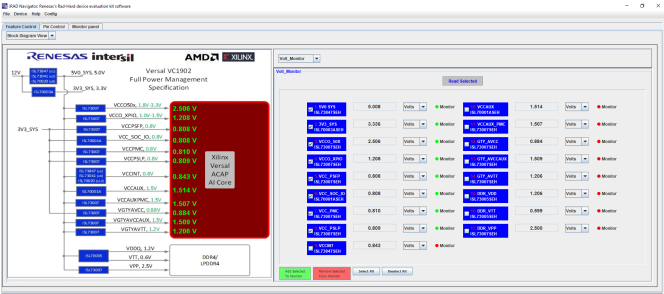
Figure 12. iRADNavigator Voltages Ready for Display in Monitor Panel
