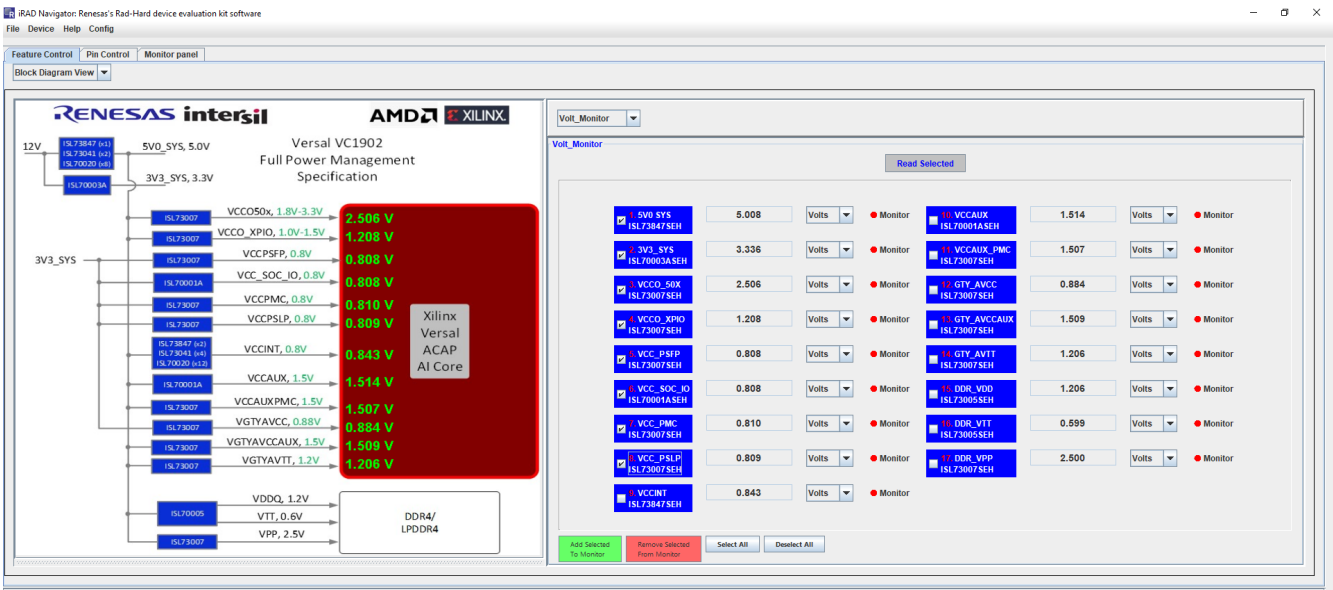
Figure 9. iRADNavigator Voltage Selection Main Screen
