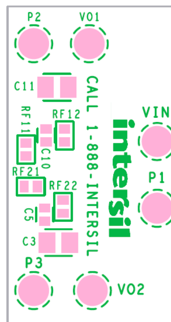
FIGURE 5. BOTTOM SILK SCREEN
