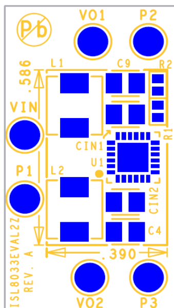
FIGURE 4. TOP COMPONENTS
