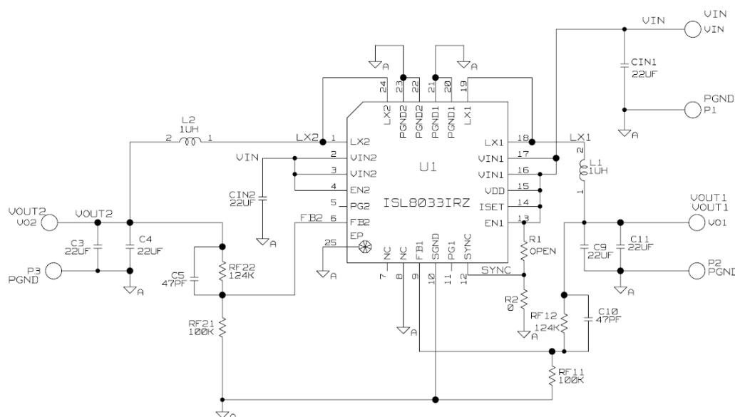
FIGURE 1. ISL8033DEMO1Z SCHEMATIC
