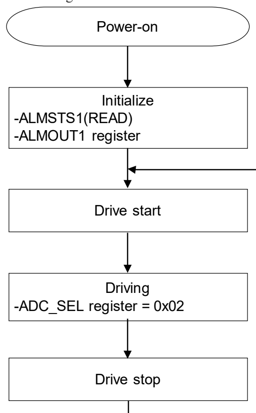
Figure 2-27 Flowchart: TSD
