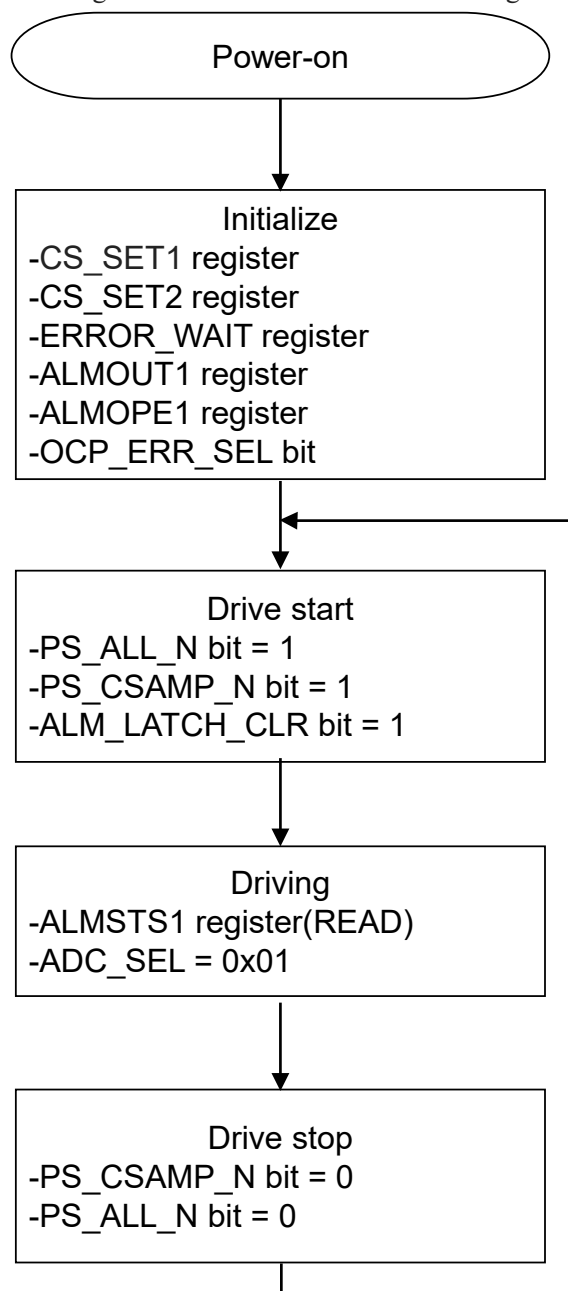
Figure 2-17 Flowchart: CS AMP setting
