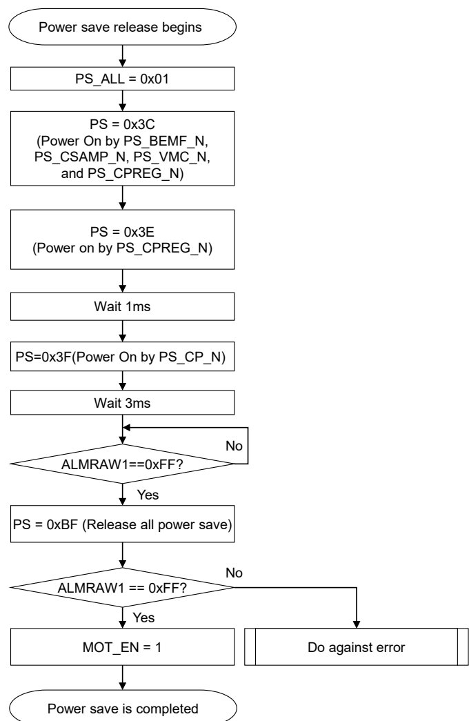
Figure 2-22 Flowchart of release power save
