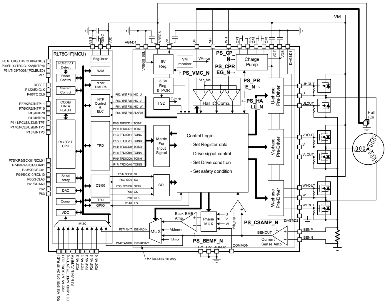
Figure 2-4 Block controlled by PS register
