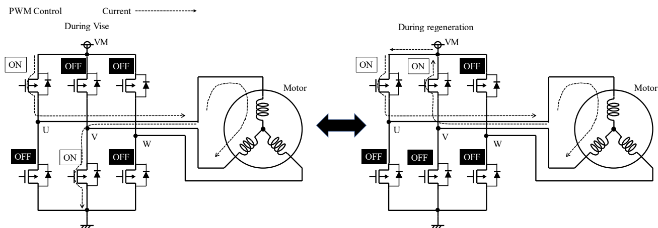
Figure 2-24 Current path of PWM control
