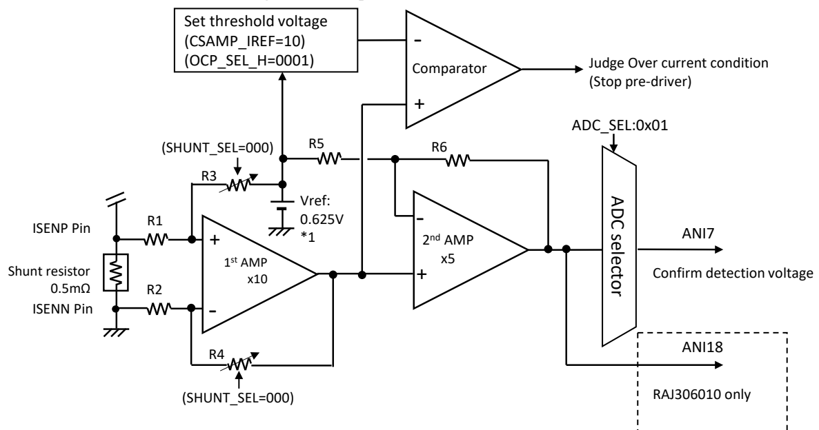
Figure 2-19 Equivalent circuit of CS AMP
