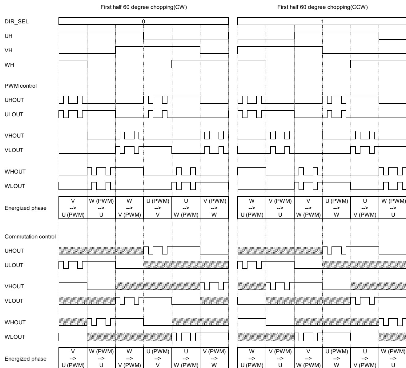
Figure 2-26 PWM control waveform and Commutation control waveform
