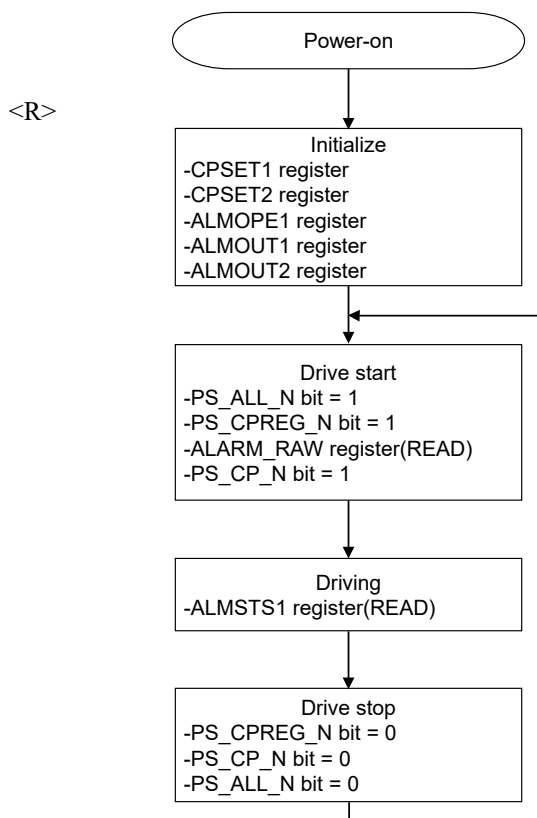
Figure 2-21 Flowchart: Charge pump
