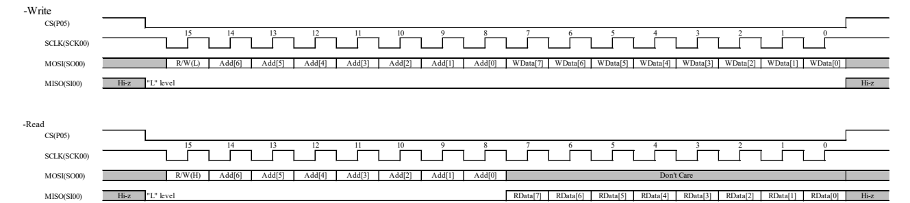
Figure 2-3 Communication format
