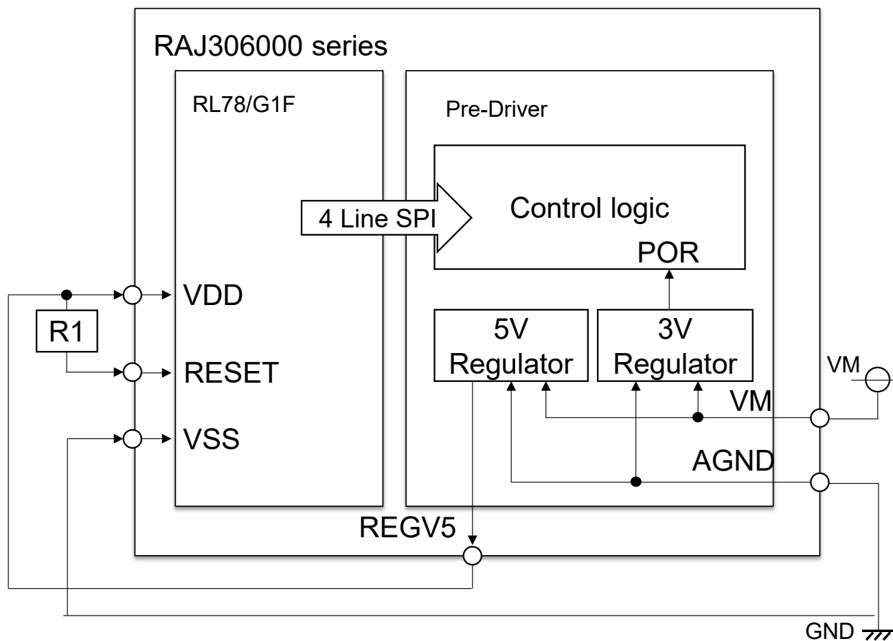
Figure 1-3 Reset Construction.
