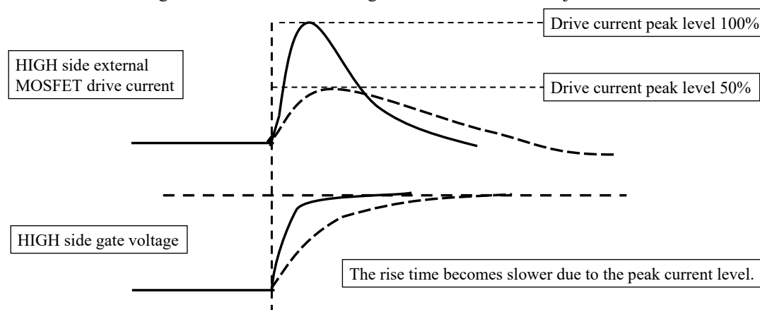
Figure 2-10 Slew Rate Change with Peak Current Adjustment
