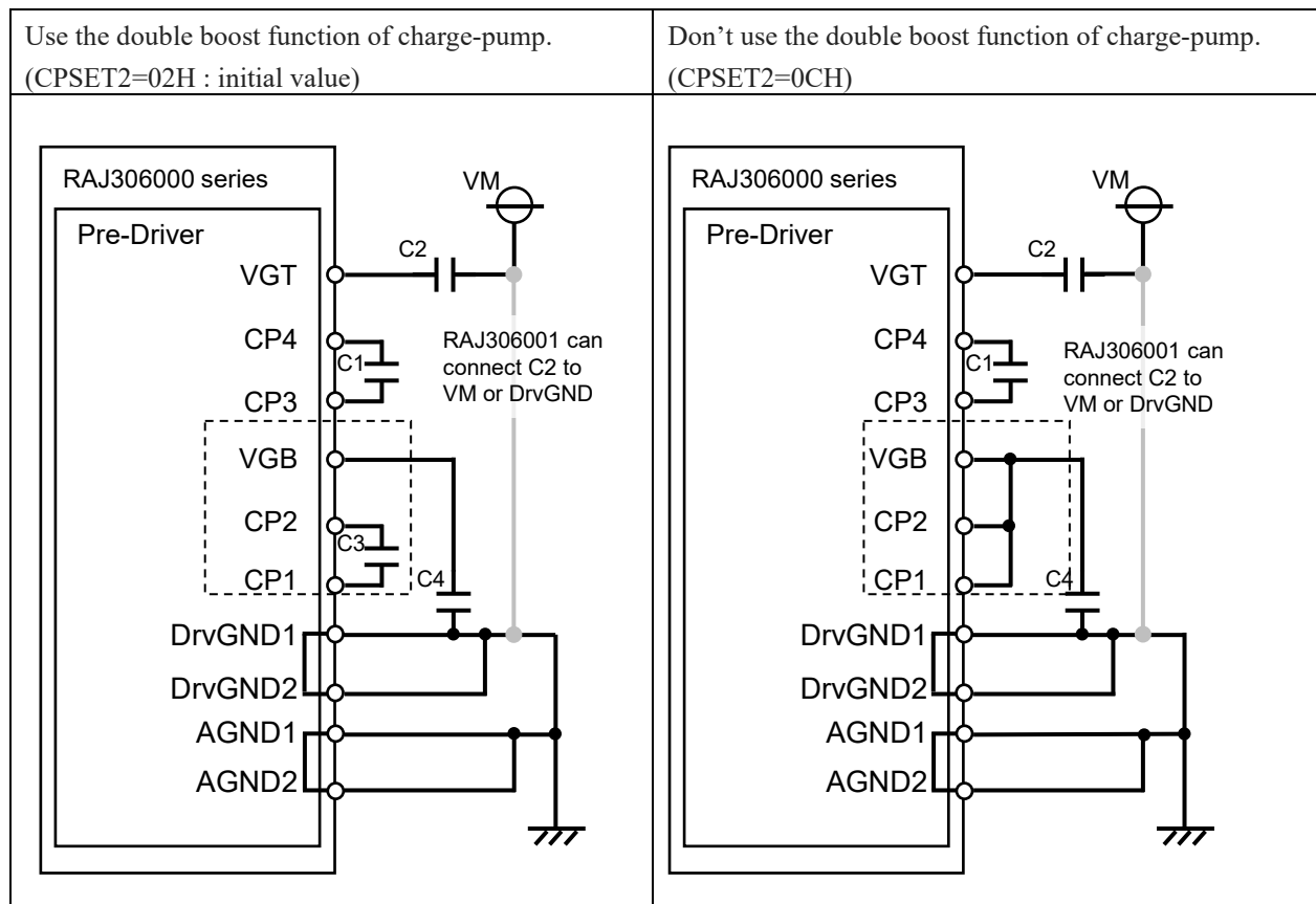
Figure 1-4 Boost function of charge-pump and recommended circuit.
