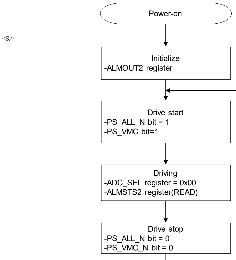
Figure 2-31 Flowchart: VMC
