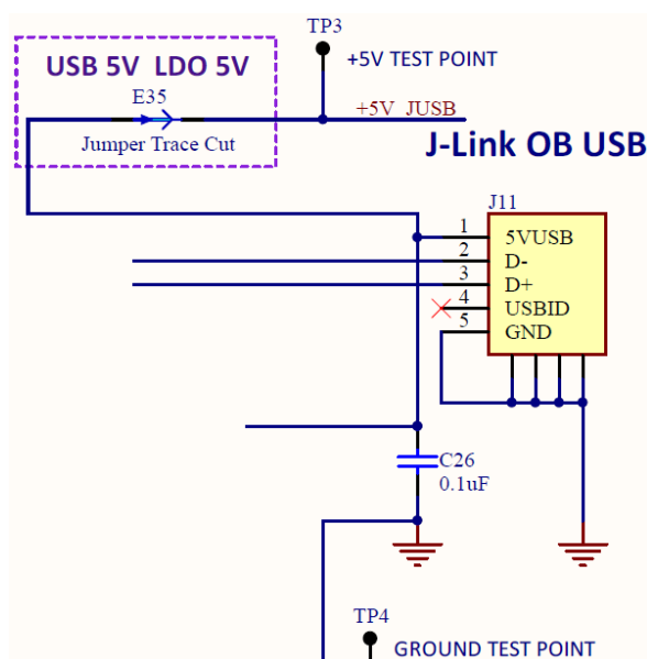
Figure 8. 5 V Power Input Circuit
