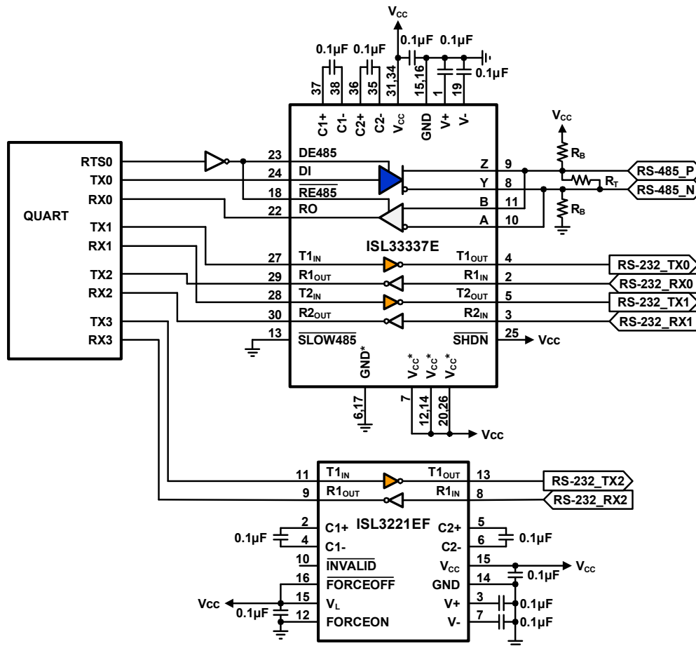
Figure 3. Single Fixed-Port ISL33337 Device Plus Single RS-232 Transceiver Allowing the Same Configuration but at Half the Cost
