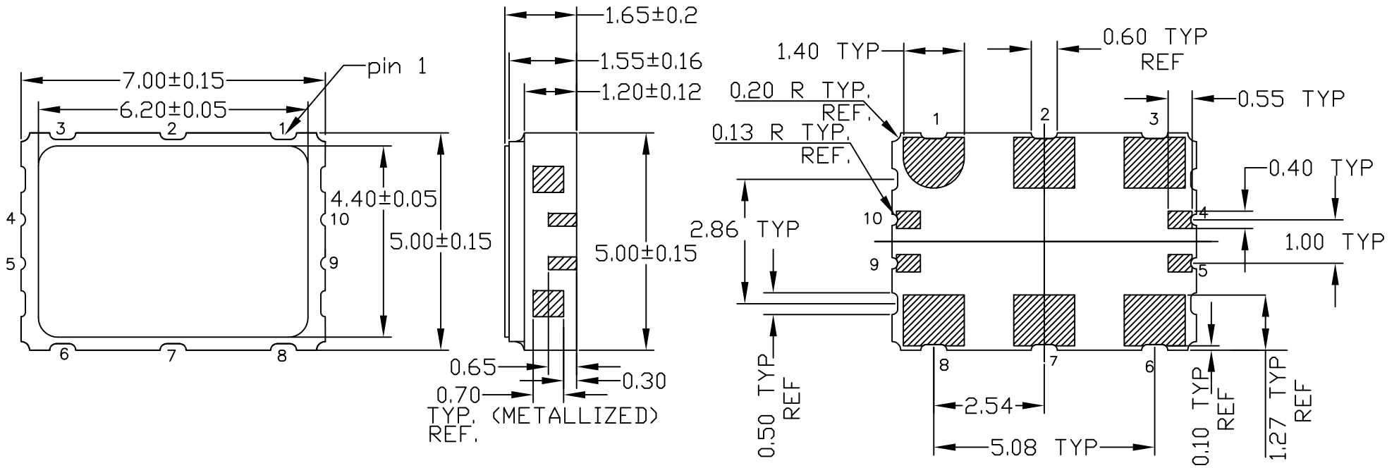
SIDE VIEW
