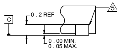
DETAIL "X"
