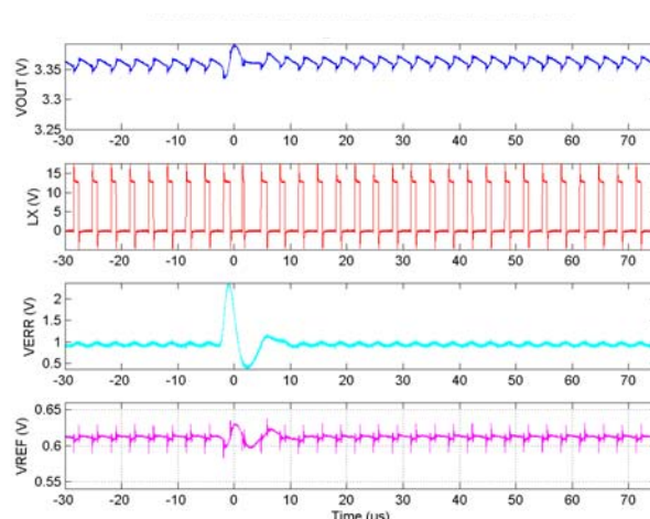
FIGURE 21. POSITIVE SET, RUN 217 CAPTURE 117, V_{IN} = 13.2V
