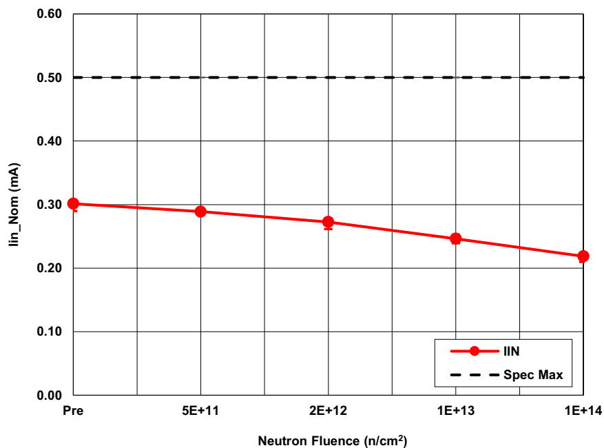
Figure 2. ISL71091SEH33 supply current ( I_{IN} ), following irradiation to each neutron fluence level. The error bars, if visible, represent the minimum and maximum measured values. The post-irradiation SMD limit is 0.5mA maximum.
