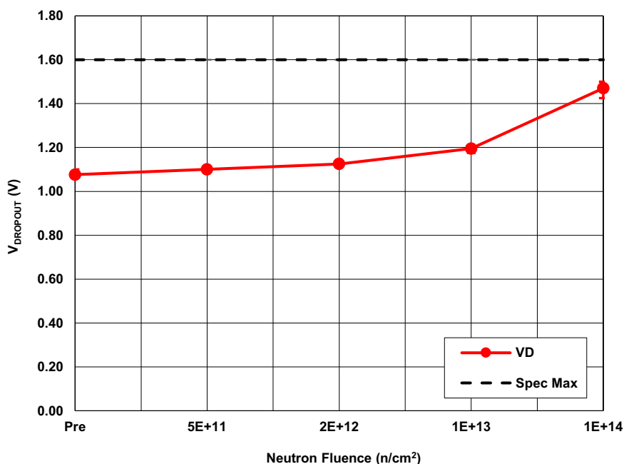
Figure 6. ISL71091SEH33 dropout voltage ( V_D ), following irradiation to each neutron fluence level. The error bars, if visible, represent the minimum and maximum measured values. The post-irradiation SMD limit is 1.6V maximum.
