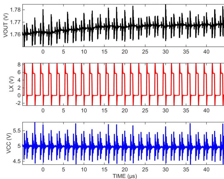
Figure 7. Example SET capture at LET = 45.8MeV·cm 2 /mg
