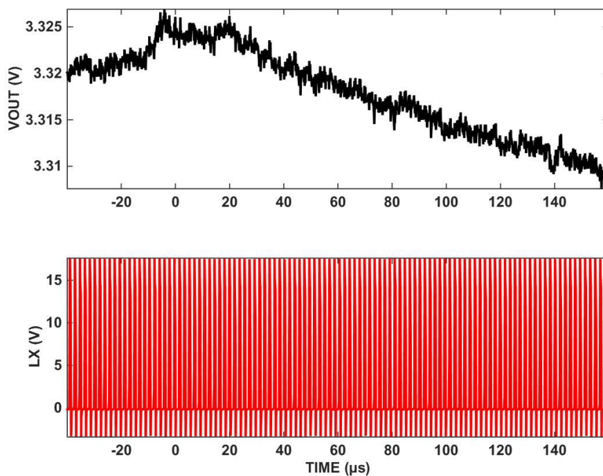
Figure 5. SET at V_{\text{OUT}} = 3.3\text{V} SET Testing
