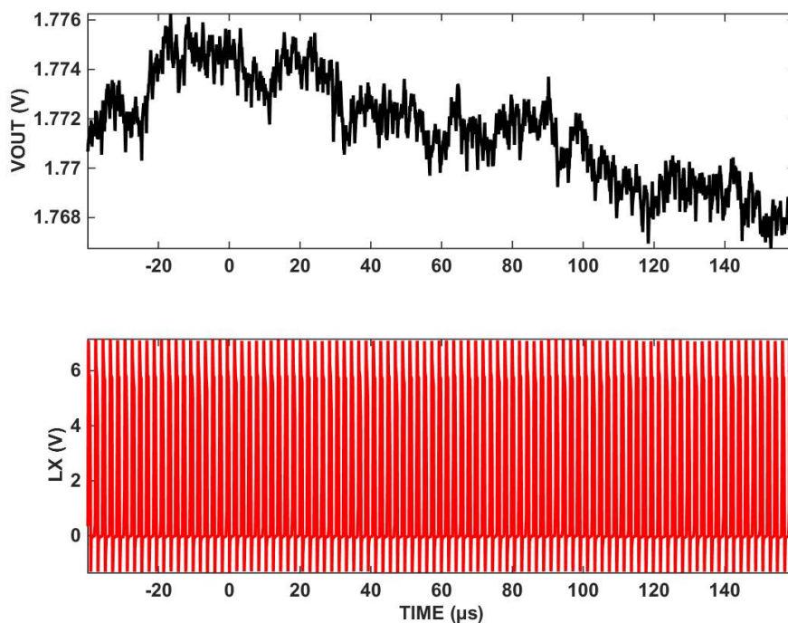
Figure 4. SET at V_{\text{OUT}} = 1.8\text{V} SET Testing
