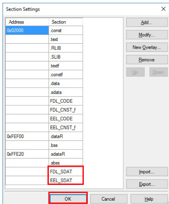
Figure 8-4. Example of Section Settings for EEPROM Emulation Library when Using CS+ (RAM Area)
