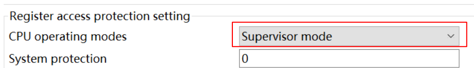
Figure 6-6. CPU operating mode after reloading in Smart Configurator for RH850 V1.6.0
