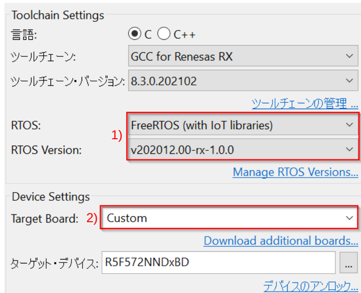
Figure 1. Project generation for FreeRTOS with Custom board (in Japanese language)
