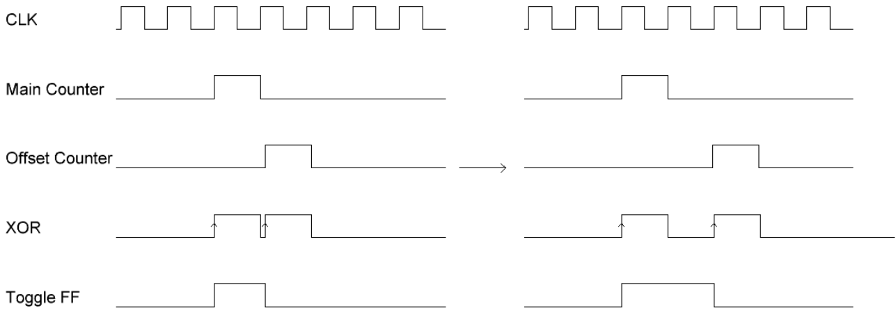
Figure 3: Counters and logic timing
