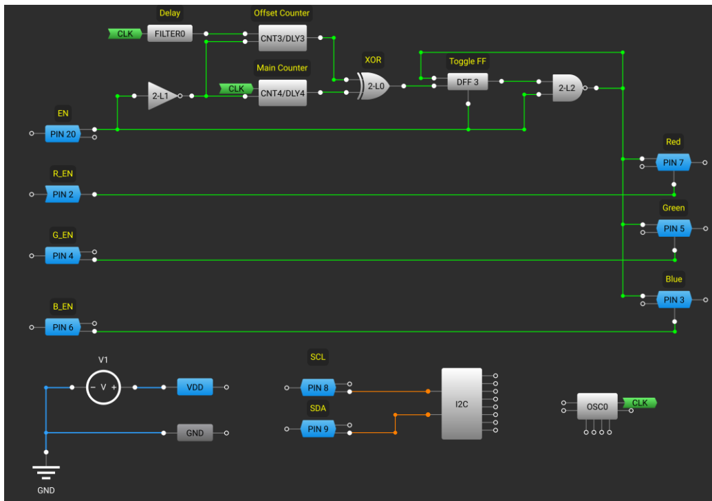
Figure 2: GreenPAK block diagram with counters for setting the PWM of each color
