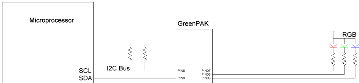
Figure 1. GreenPAK Used as an RGB Driver in a Larger System
