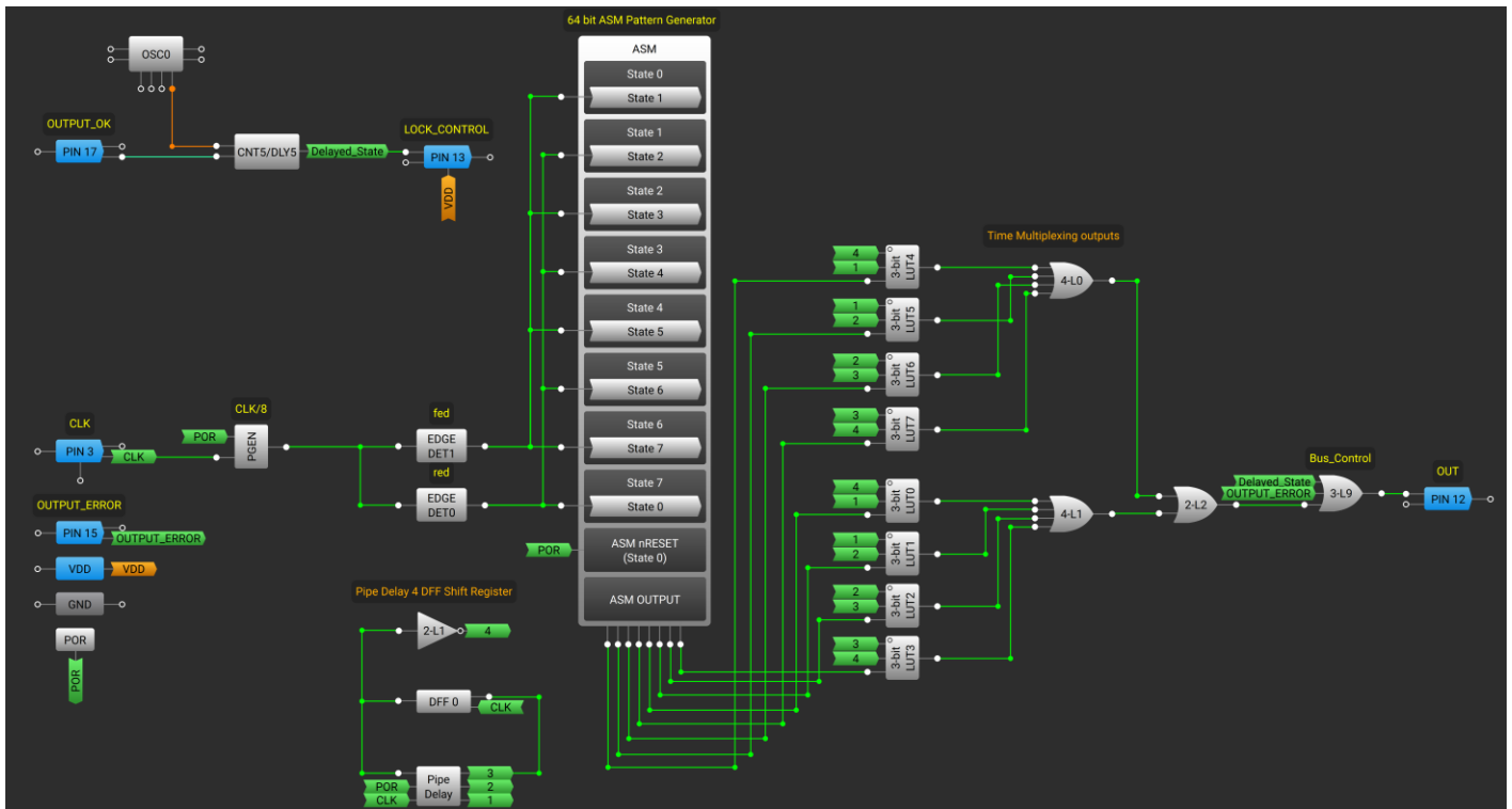
Figure 6. Configuration of the ASM's RAM table
