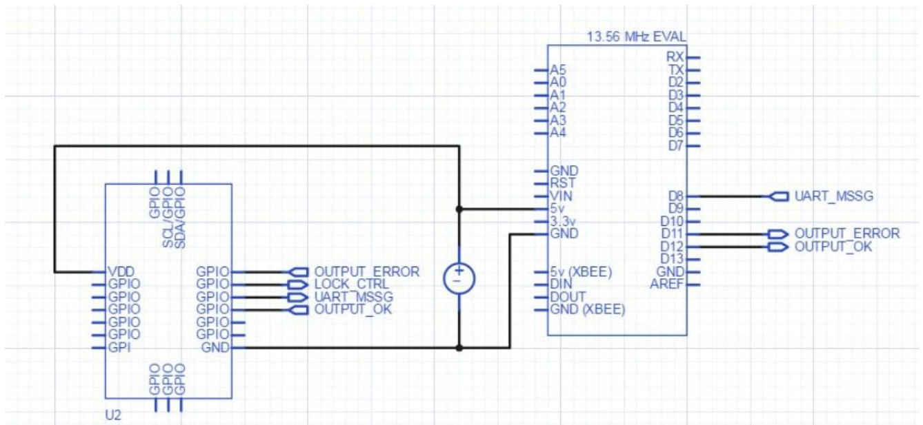
Figure 3. Schematic with SparkFun DEV10406 RFID Evaluation Shield
