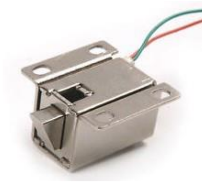
Figure 9. The lock used
