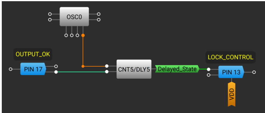
Figure 7. Creating a delay of 5 seconds to control the lock
