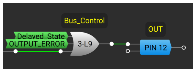
Figure 8. The Bus_Control LUT
