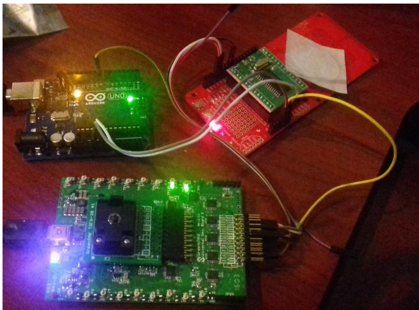
Figure 12. A tag prompts the GreenPAK to wait
