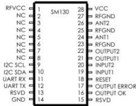
Figure 1. The SM130 RFID module
