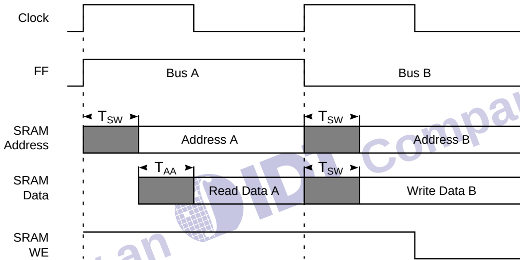
Figure 4. Time Shared Dual Port SRAM Timing Diagram
