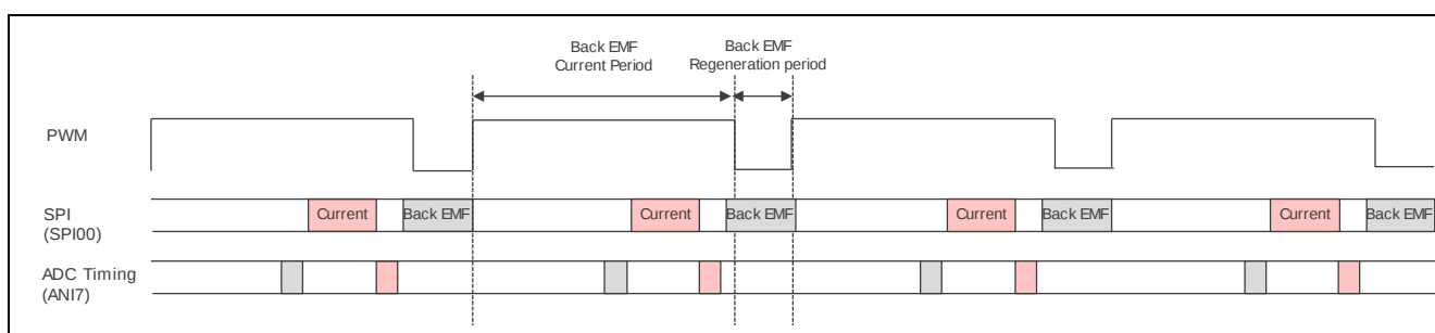
Figure 3-5 Back EMF detection (Current period) and timing of Current detection (PWM Duty \geq 50[%])
