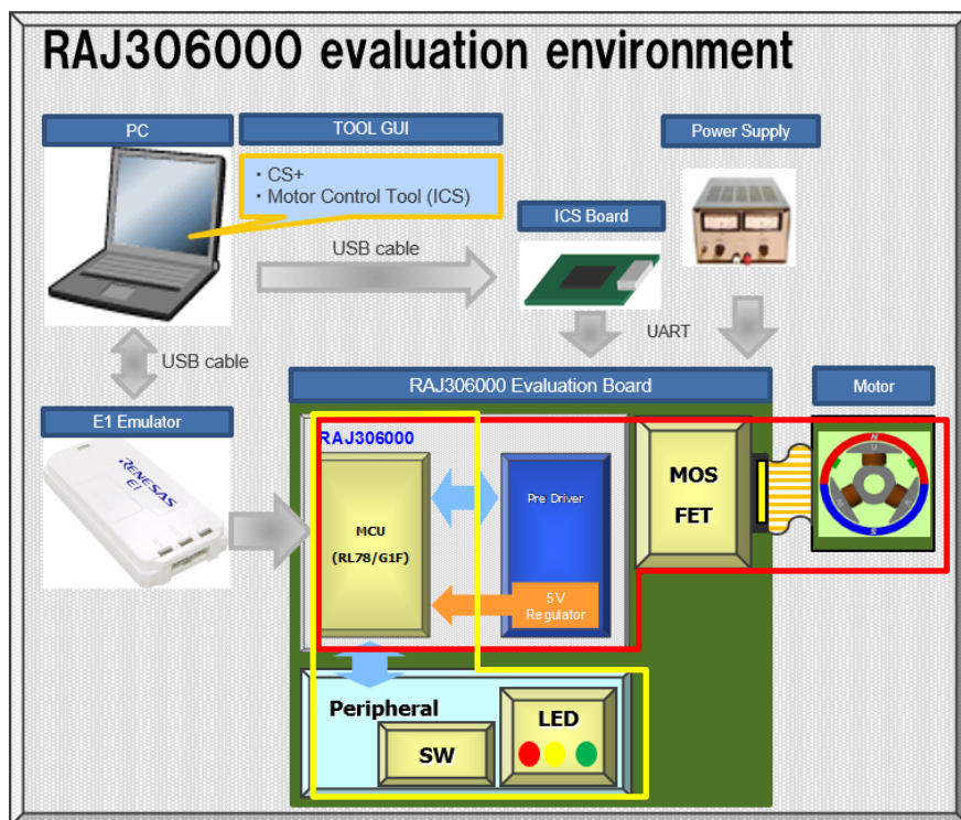
Figure 2-1 System configuration
