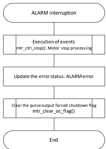
Figure 3-17 Flow chart (ALARM interruption processing)
