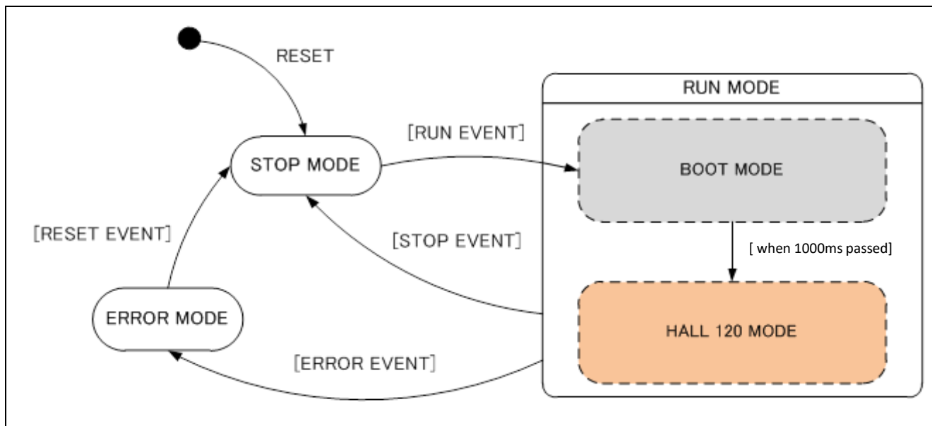
Figure 3-4 状態遷移図
