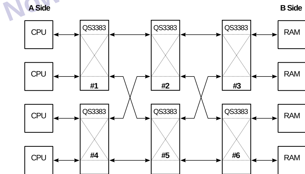
Figure 1. 4 x 4 Crossbar Using QuickSwitch
