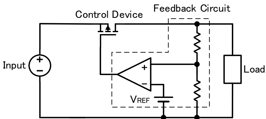
Figure 3-3 Linear regulator basic configuration
