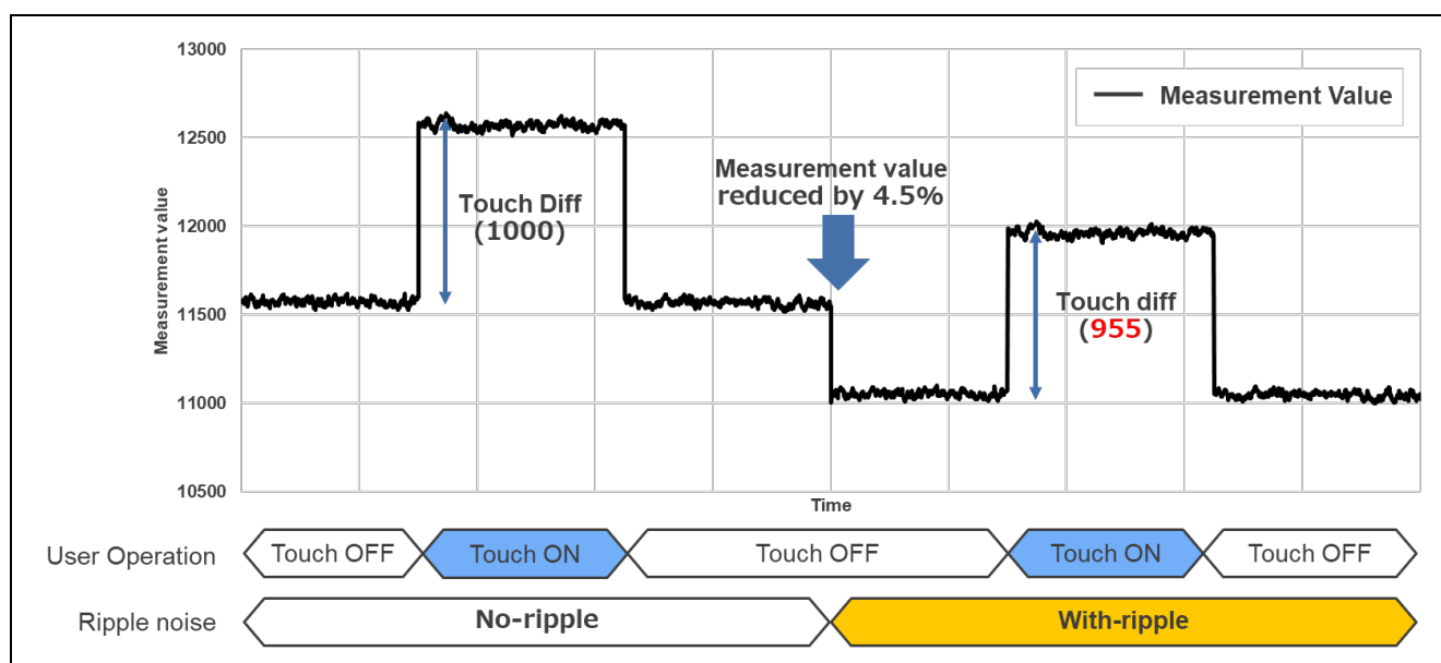
Figure 2-2 Example of measurement value deterioration due to ripples [touch difference=1000, Measurement value reduced by 4.5%]
