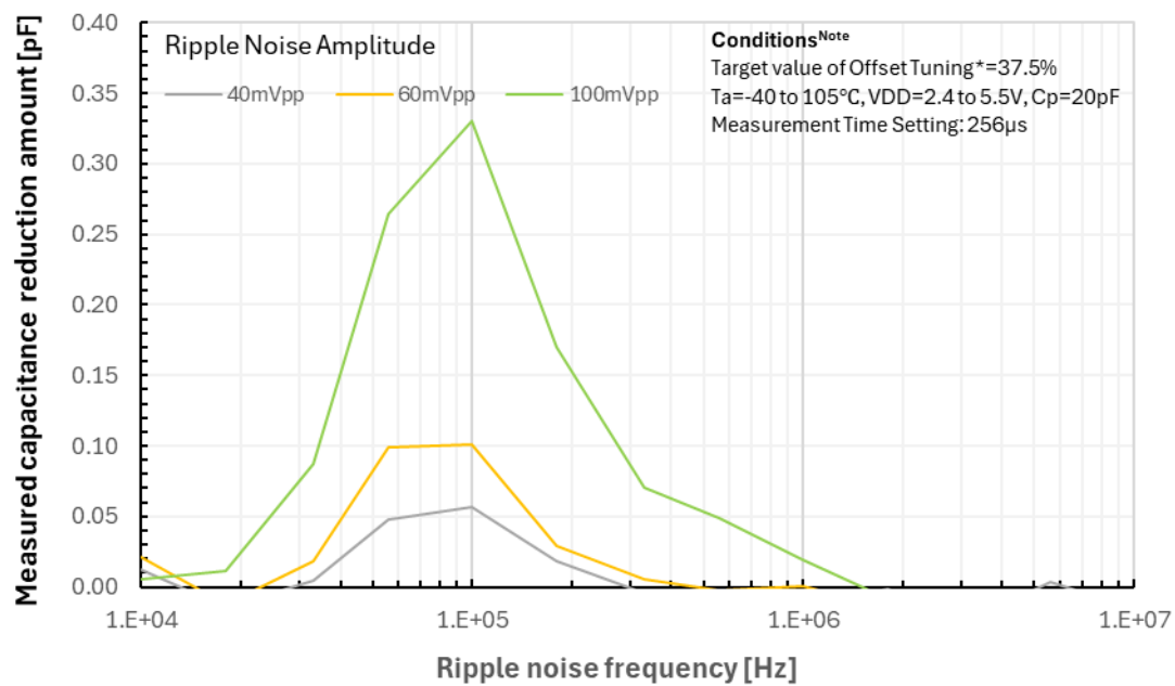
Figure 5-3 Ripple characteristic of CTSU2 (Measured Current Range = 40uA)
