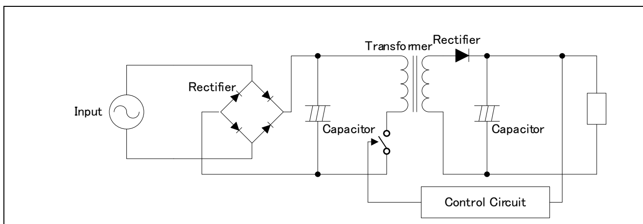
Figure 3-2 Typical configuration of switching-system AC/DC converter
