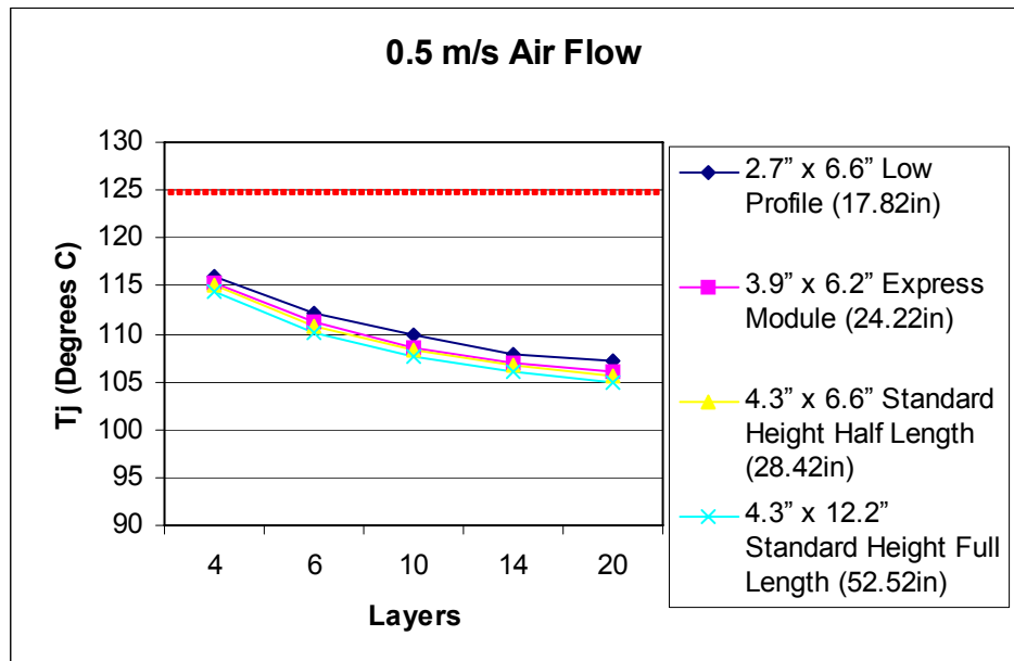
Figure 4 PES16T4G2 Heat Sink Requirements with Air Flow
