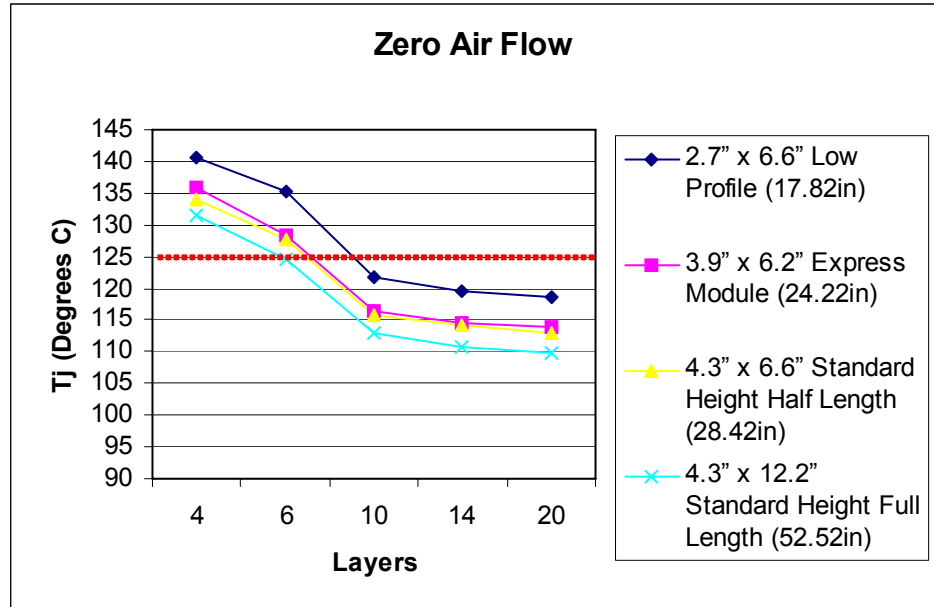
Figure 3 PES16T4G2 Heat Sink Requirements without Air Flow
