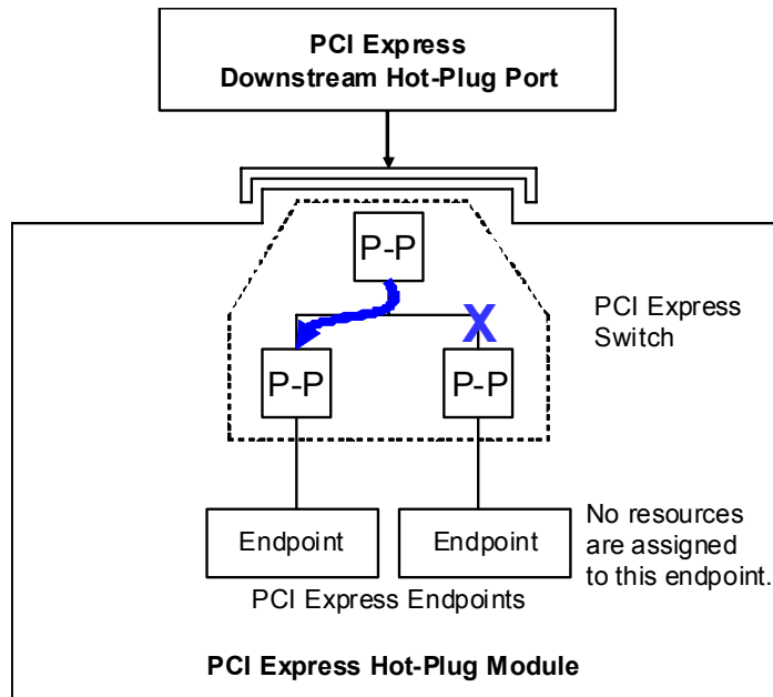
Figure 3 Bridge Resource Assignments Behind a PCIe Switch
