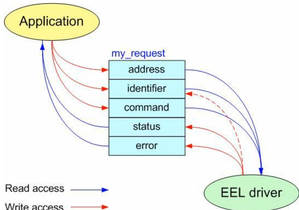
Figure 3-1 request variable synchronizing EEL and the application
