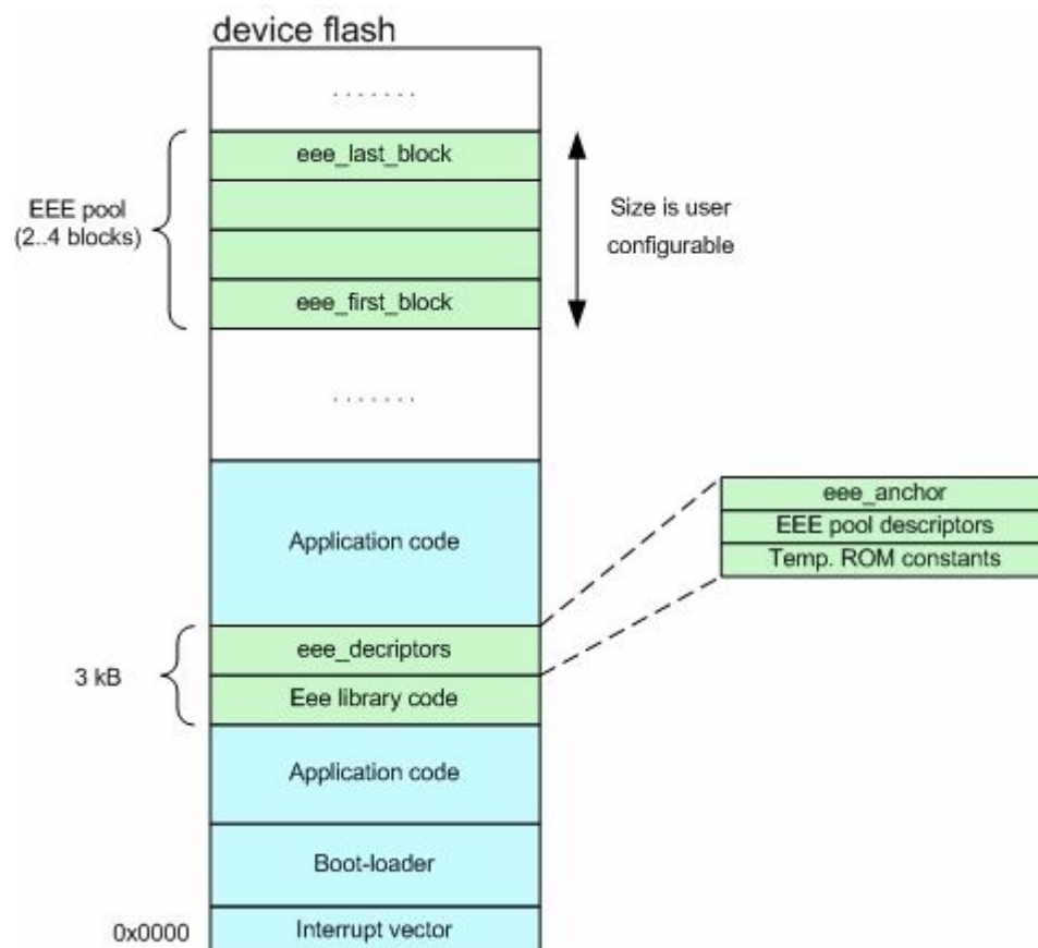
Figure 2-5 physical placement inside device flash memory
