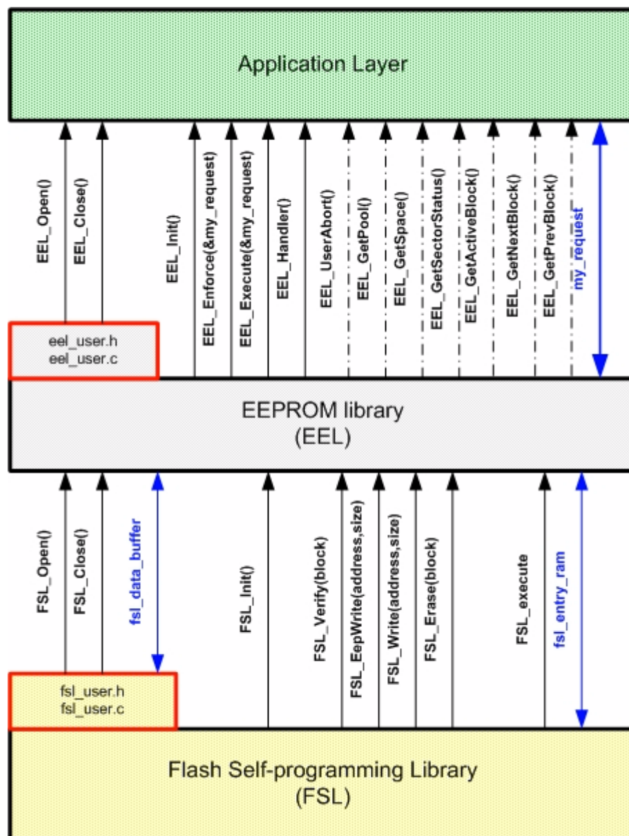
Figure 2-2 import export diagram (RAM variables marked in blue)
