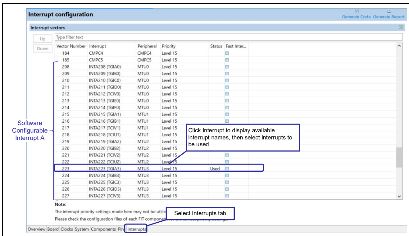
Figure 3.4 Interrupt Settings
