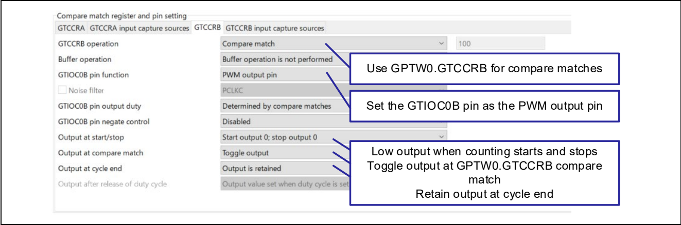
Figure 4.18 GPT0 Settings (3/3)
