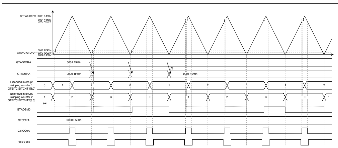
Figure 4.24 Extended Interrupt Skipping Counter 2 Operation with the Initial Value of 1
