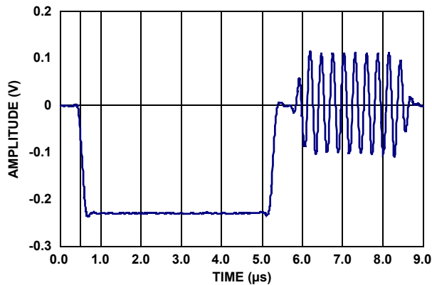
FIGURE 1. NTSC BI-LEVEL SYNC PULSE WITH COLOR BURST Another type of synchronization pulse is the tri-level sync. Analog HD video uses tri-level sync. Tri-level sync uses a negative going pulse and a subsequent positive going pulse, which is centered at the blanking level. The system uses the midpoint of the low to high transition (or zero crossing) to trigger the start of a video line. Unlike the bi-level sync that introduces a DC offset due to a negative going pulse, tri-level sync has a net DC offset value of zero. This effectively reduces some issues during signal processing and helps to more accurately synchronize the components of an HD video signal. Figure 2 depicts a tri-level sync pulse from a 1080i/30 HD video waveform.
