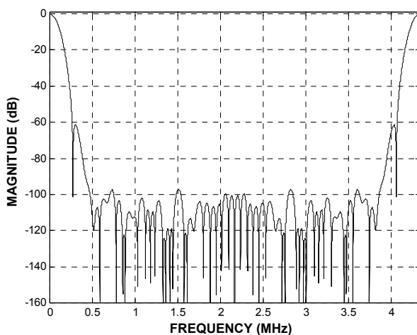
FIGURE 8. SHAPING FILTER FREQ. RESPONSE
