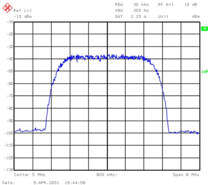
FIGURE 58. ANALOG SPECTRUM
