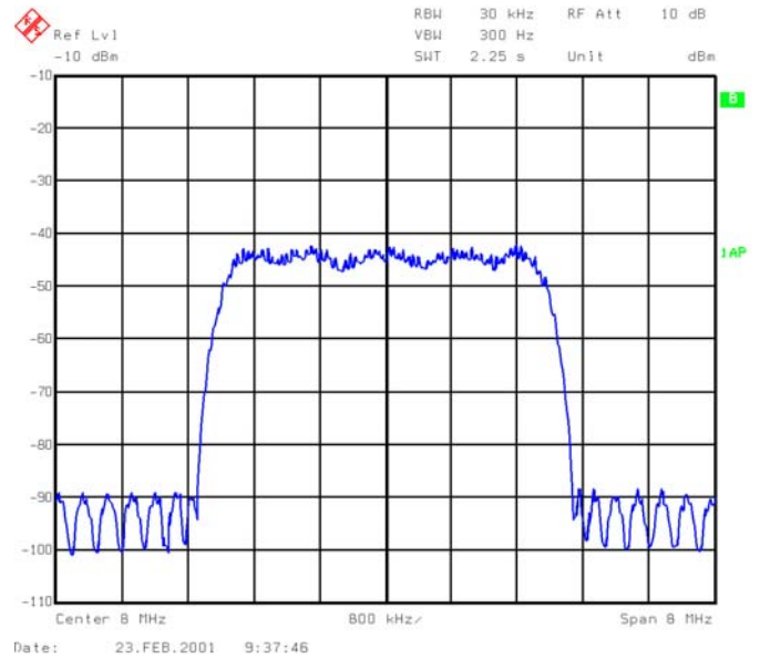
FIGURE 48. ANALOG SPECTRUM
