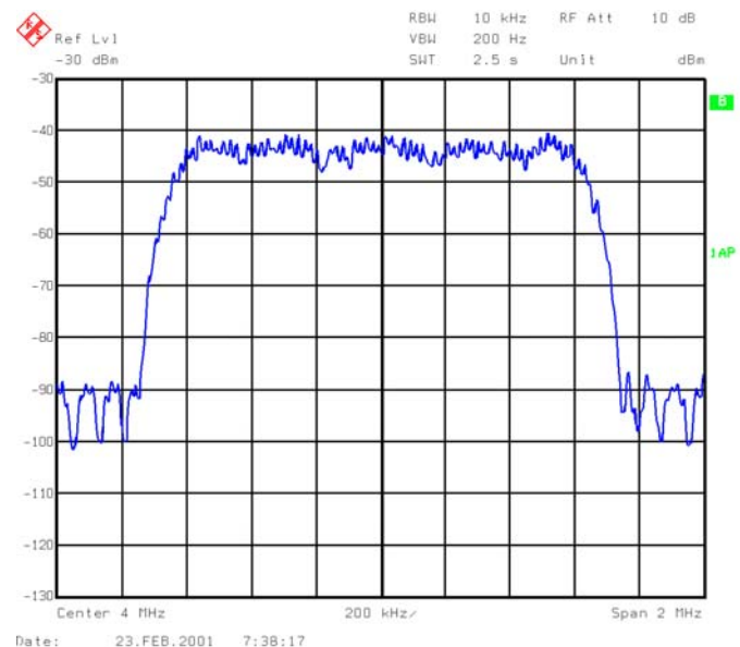
FIGURE 38. ANALOG SPECTRUM
