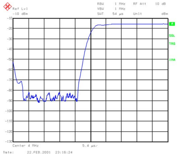
FIGURE 30. GSM RAMP UP TIMING
