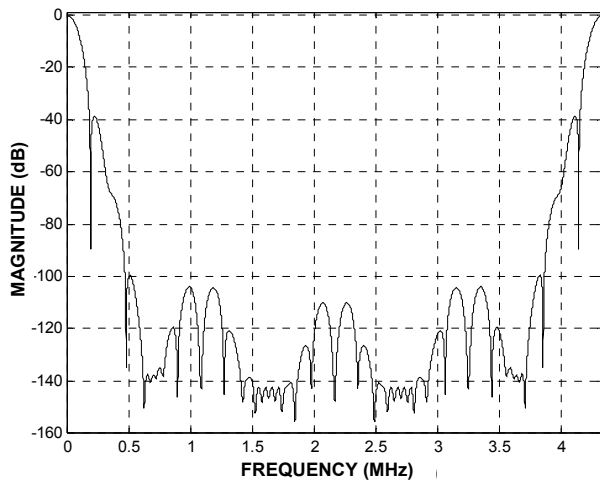
FIGURE 19. SHAPING FILTER FREQ. RESPONSE
