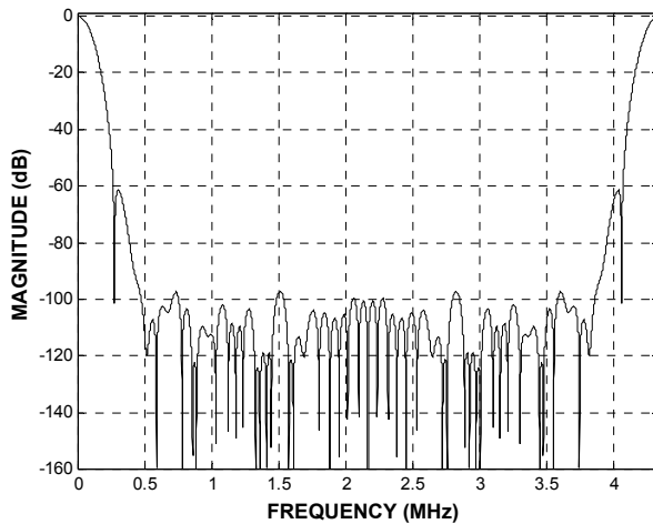
FIGURE 3. SHAPING FILTER FREQUENCY RESPONSE
