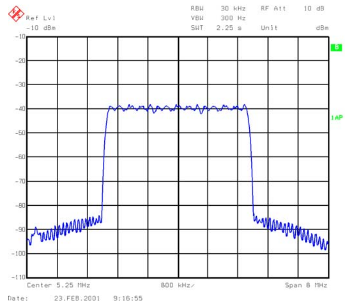
FIGURE 42. ANALOG SPECTRUM
