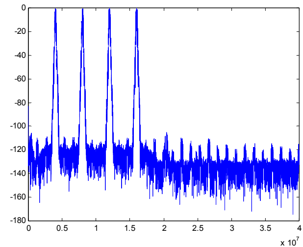
FIGURE 6. DIGITAL OUTPUT
