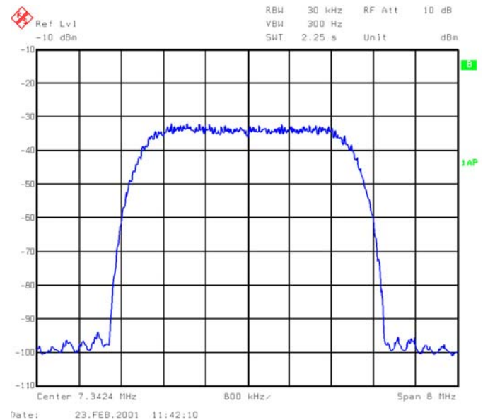
FIGURE 52. ANALOG SPECTRUM
