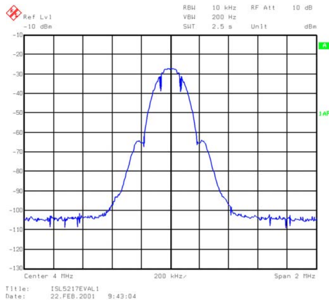
FIGURE 4. ANALOG SPECTRUM
