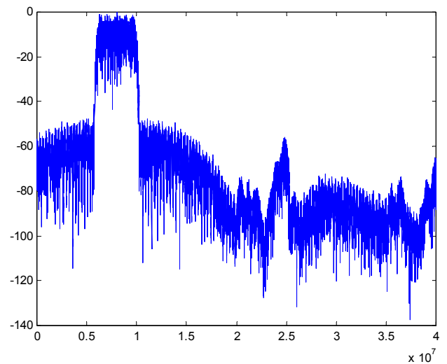
FIGURE 49. DIGITAL OUTPUT
