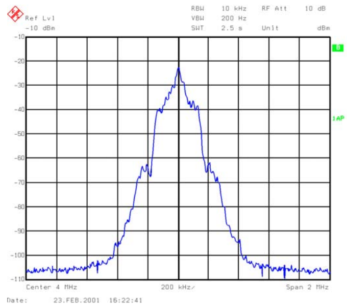
FIGURE 9. ANALOG SPECTRUM
