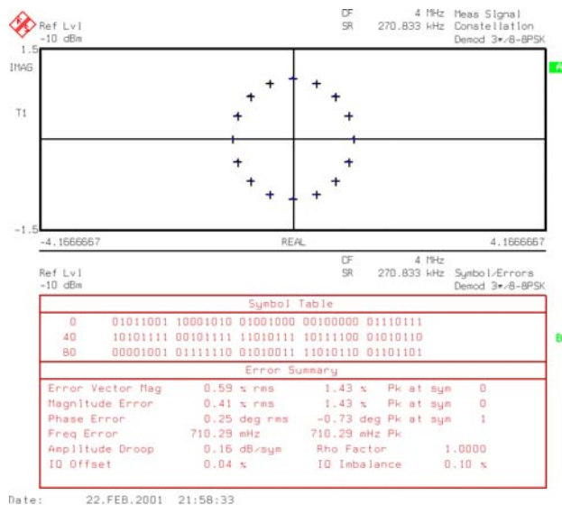
FIGURE 16. VECTOR ANALYZER OUTPUT
