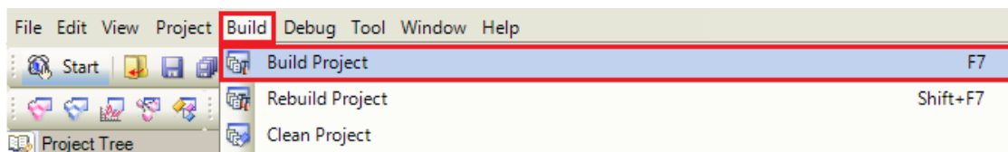
Figure 3.3 Build (CS+)
