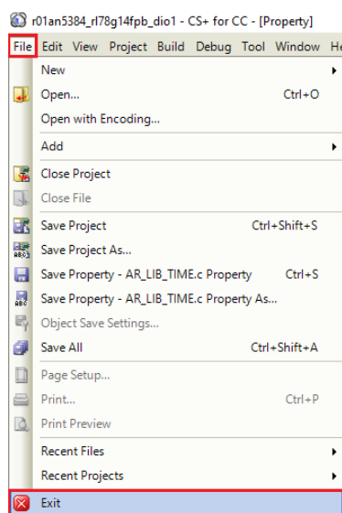
Figure 3.10 Exit CS+
