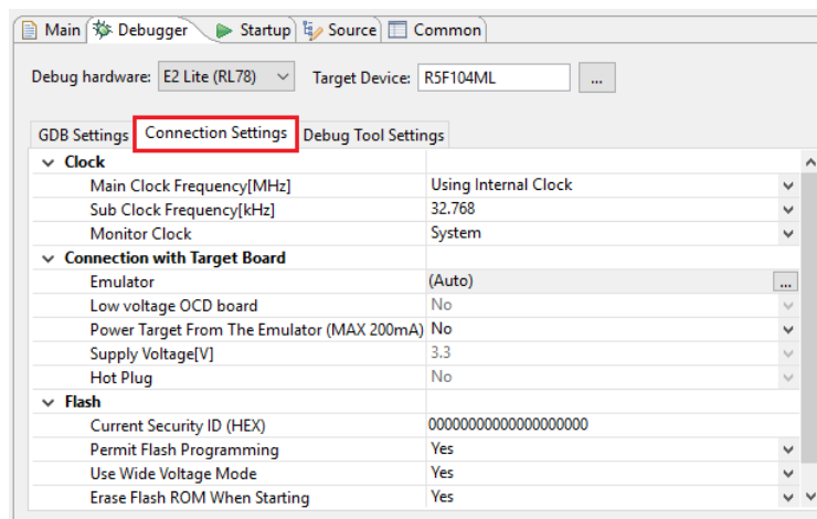
Figure 3.28 "Connection Settings" tab settings
