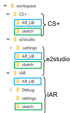
Figure 2.1 Folder configuration
