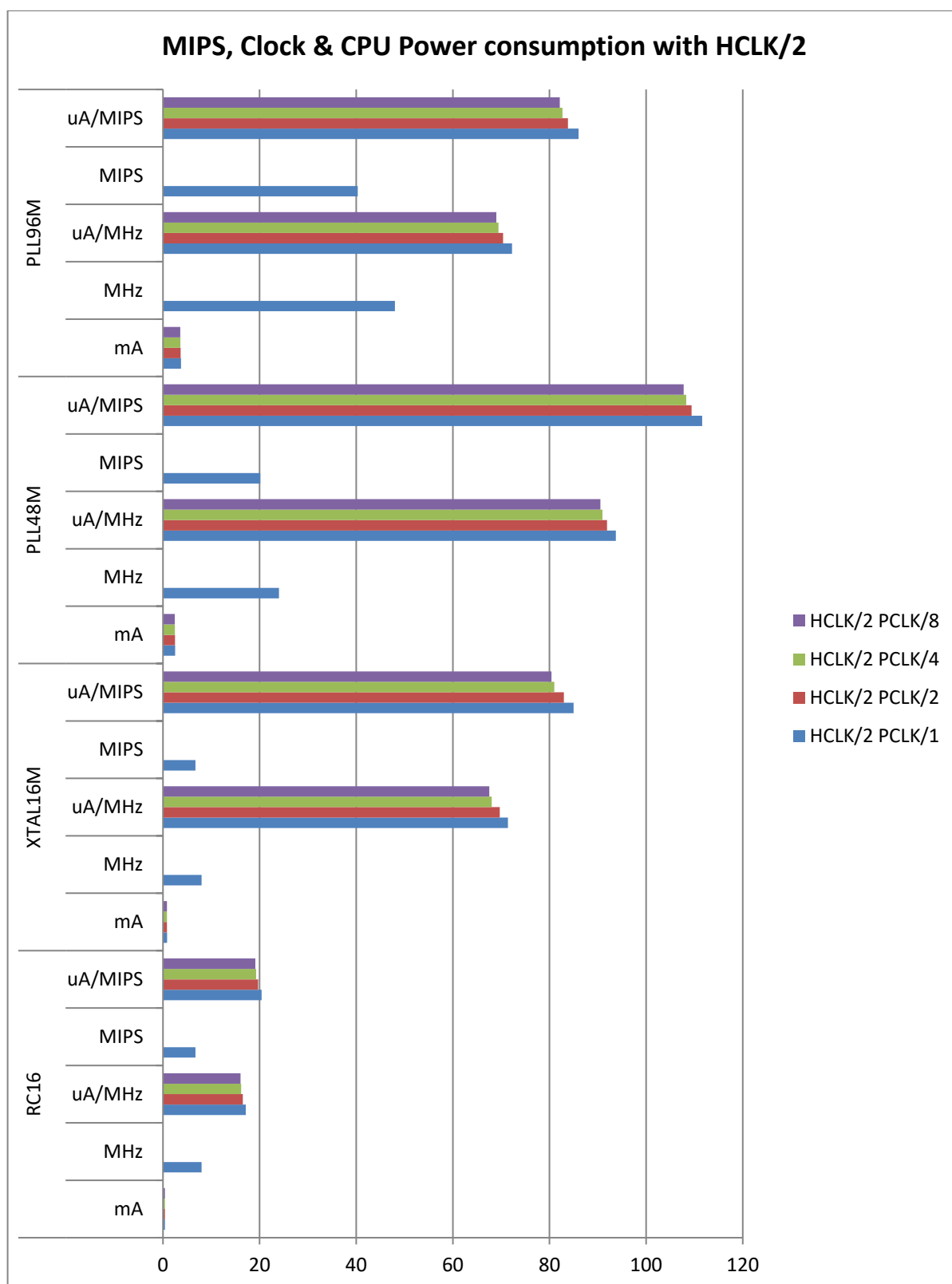
Figure 8: MIPS, Clock &amp; CPU Power consumption with HCLK/2
