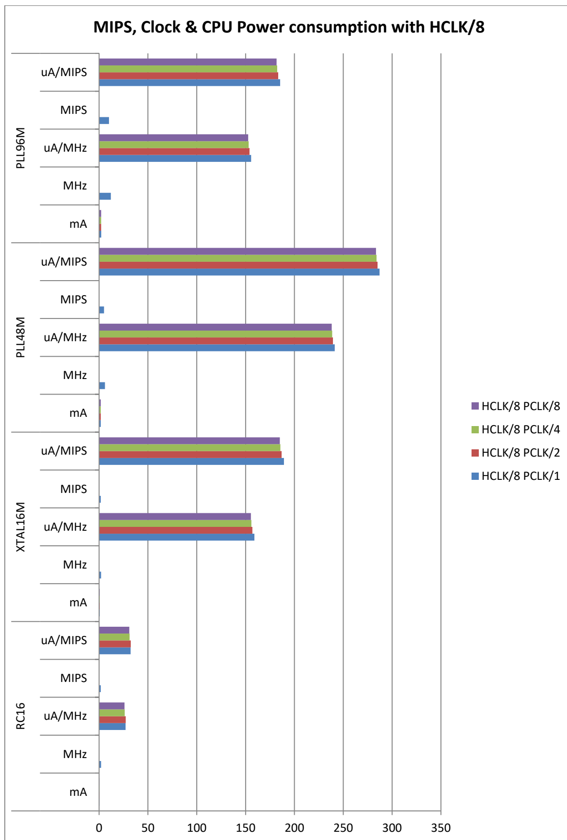
Figure 10: MIPS, Clock &amp; CPU Power consumption with HCLK/8
