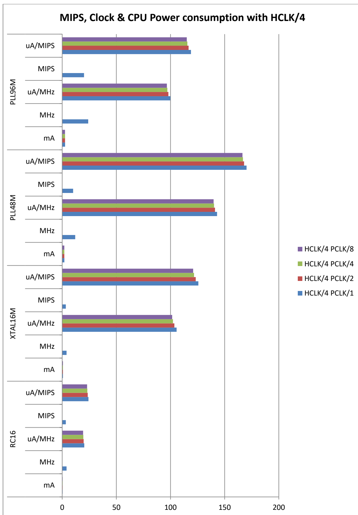
Figure 9: MIPS, Clock &amp; CPU Power consumption with HCLK/4
