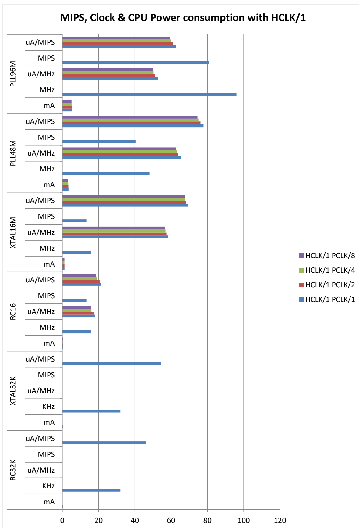
Figure 7: MIPS, Clock &amp; CPU Power consumption with HCLK/1
