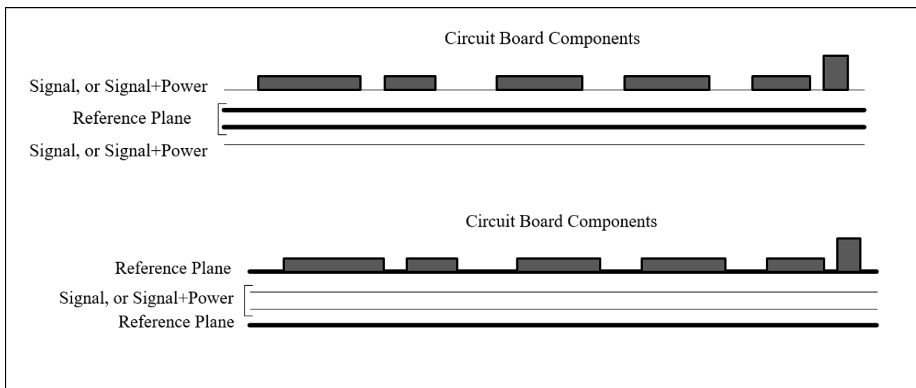
Figure 7. 4-Layer Design
