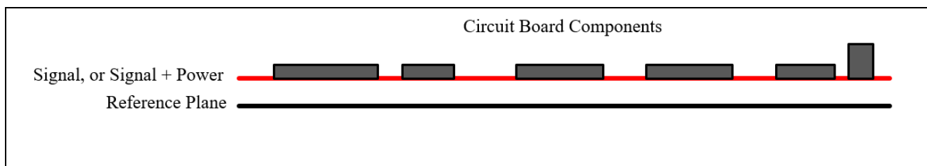
Figure 6. 2-Layer Design
