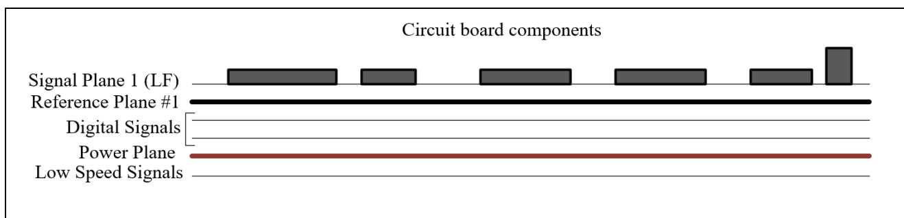
Figure 8. 6-Layer Design
