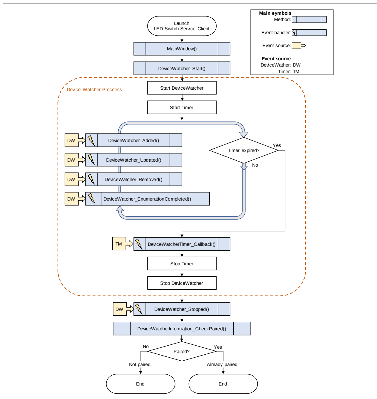
Figure 4-1 Flowchart of Launch application
