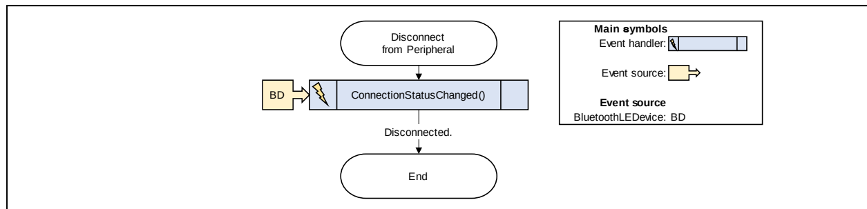
Figure 4-16 Flowchart of Disconnect from evaluation board
