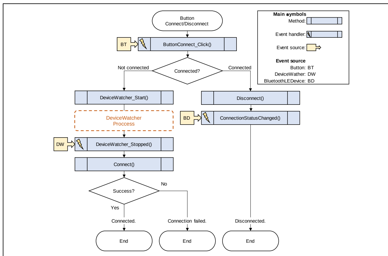
Figure 4-4 Flowchart of Connect/Disconnect button
